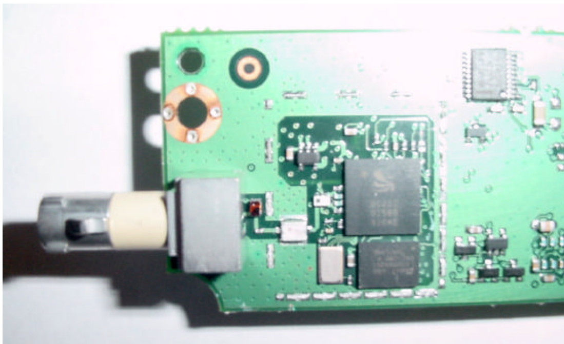
Figure 5. Close-up image of the BT circuit without the RF shield. The design is based on BC02-External Flash chip-set from Cambridge Silicon Radio. Topside view is shown in this picture.
