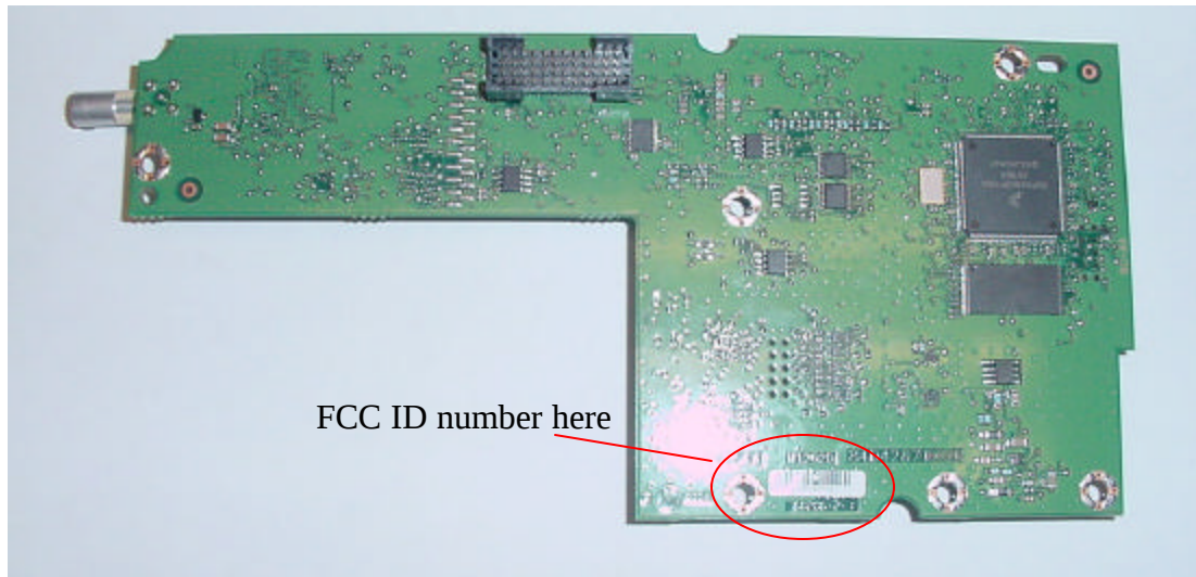
Figure 6. Internal bottom-side view of the of the BlueTooth module TCU1P03_m1202d. Internal label with FCC ID number will be placed onto the bottom side of the pcb in the location shown in the picture.
