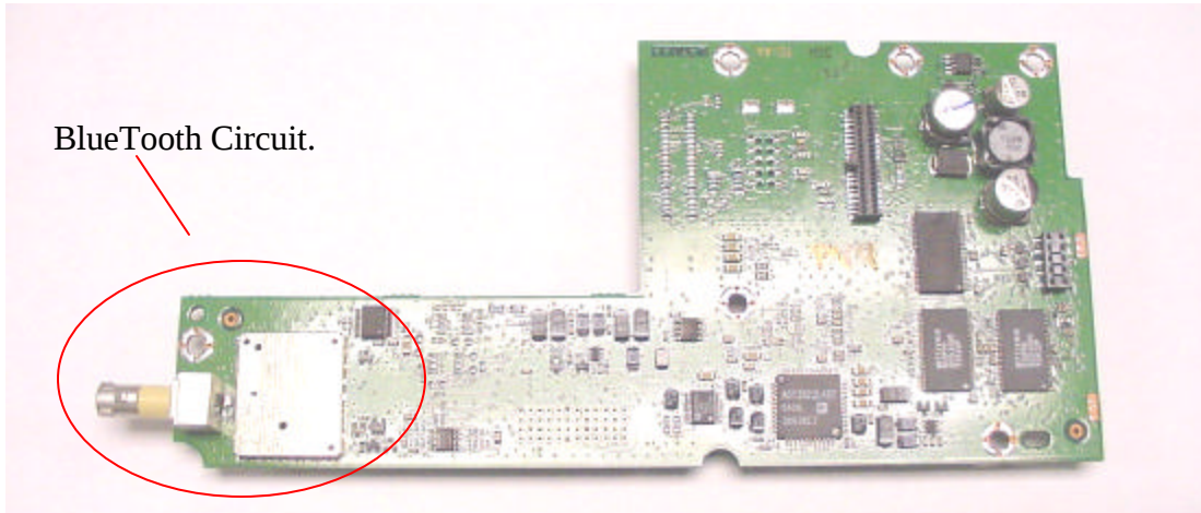
Figure 4. Internal topside view of the Bluetooth module TCU1P03_m1202d. The Bluetooth circuit is integrated onto a pcb that is shared with the TCU.
