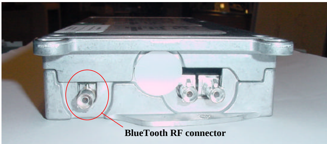
Figure 2. External side view of a fully assembled TCU with the BlueTooth connector shown. An external BT antenna will be attached to the connector during BMW factory assembly process.
