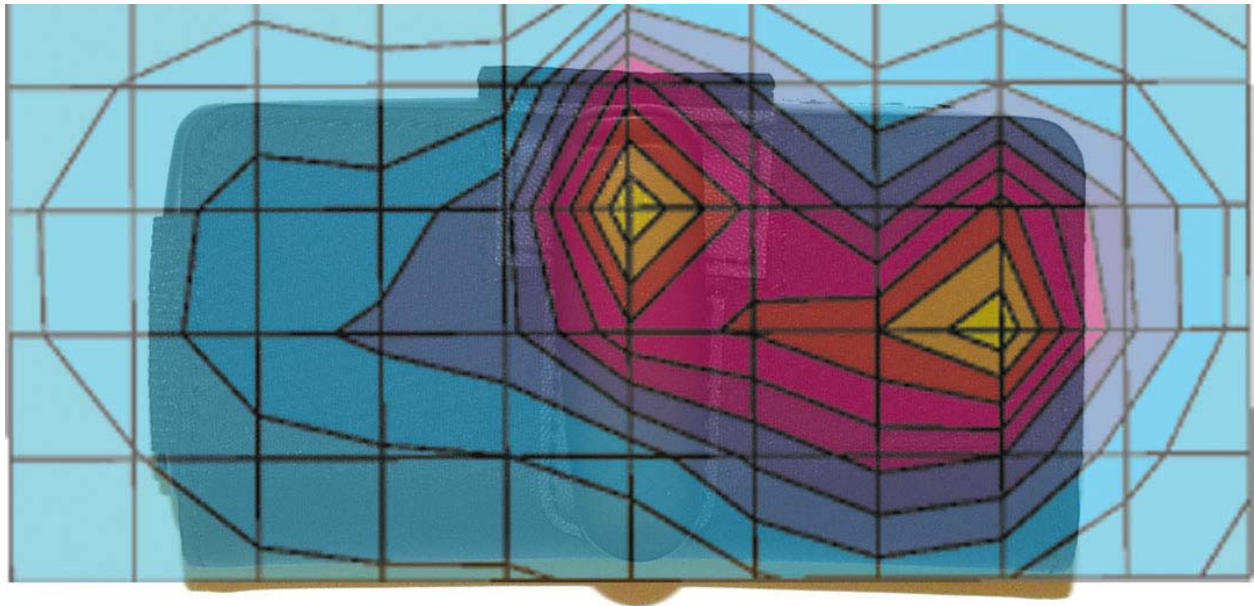
Figure 3. Typical 1900 MHz Body-Worn Contour Overlaid on Phone
