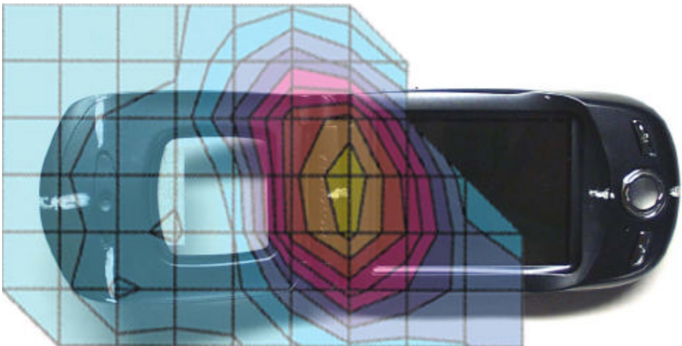
Figure 2. Typical 1900MHz Left Head Adjacent Contour Overlaid on Phone with Antenna Fixed (15 ° Tilt)
