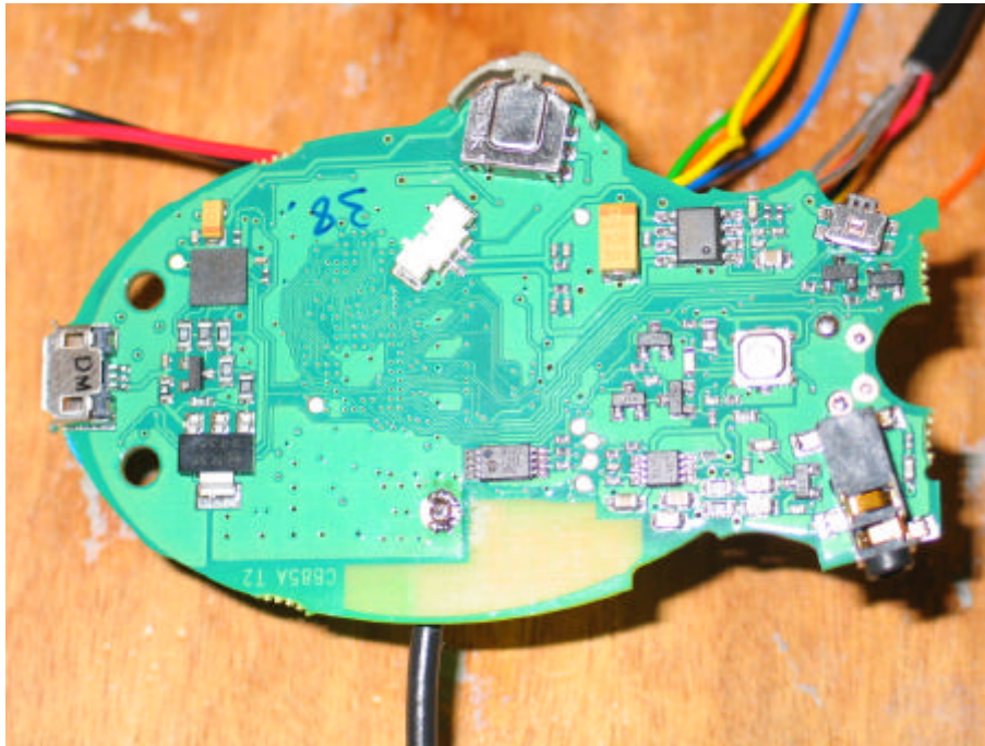
Picture 3 : EUT (view to the PCB bottom side)
