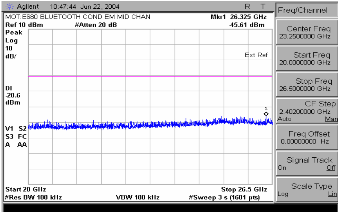
Conducted Spurious Emissions 20-26.5GHz (Mid Chan Enabled)
