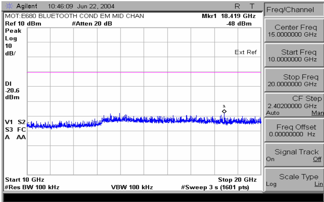
Conducted Spurious Emissions 10-20GHz (Mid Channel Enabled)
