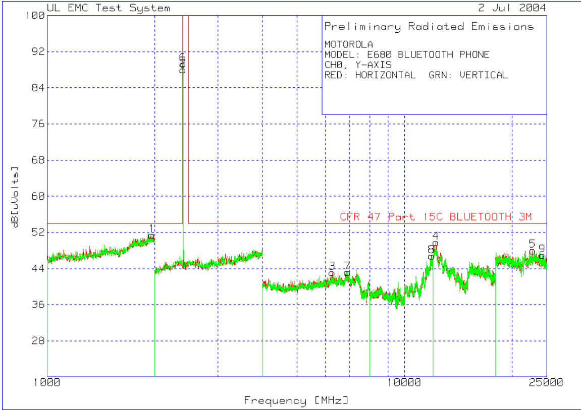
1-25GHz Low Channel Y-Orientation
