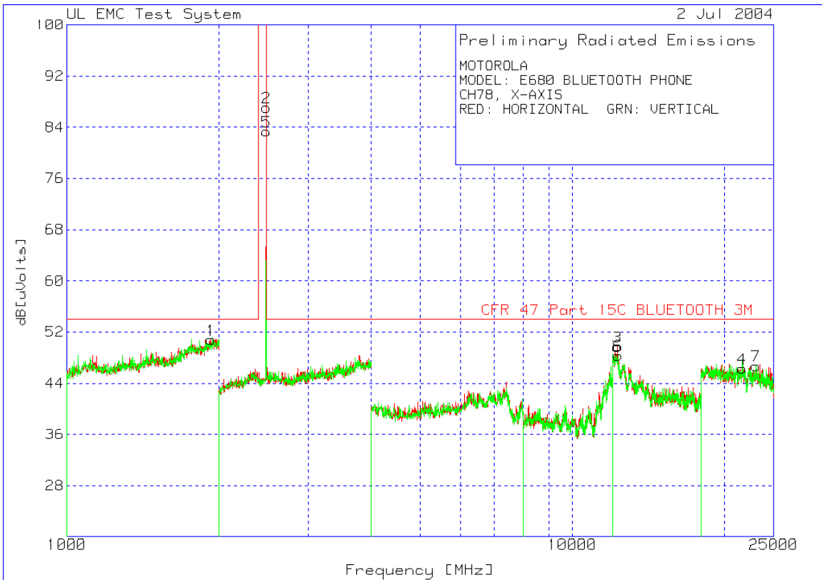
1-25GHz High-Channel X-Orientation
