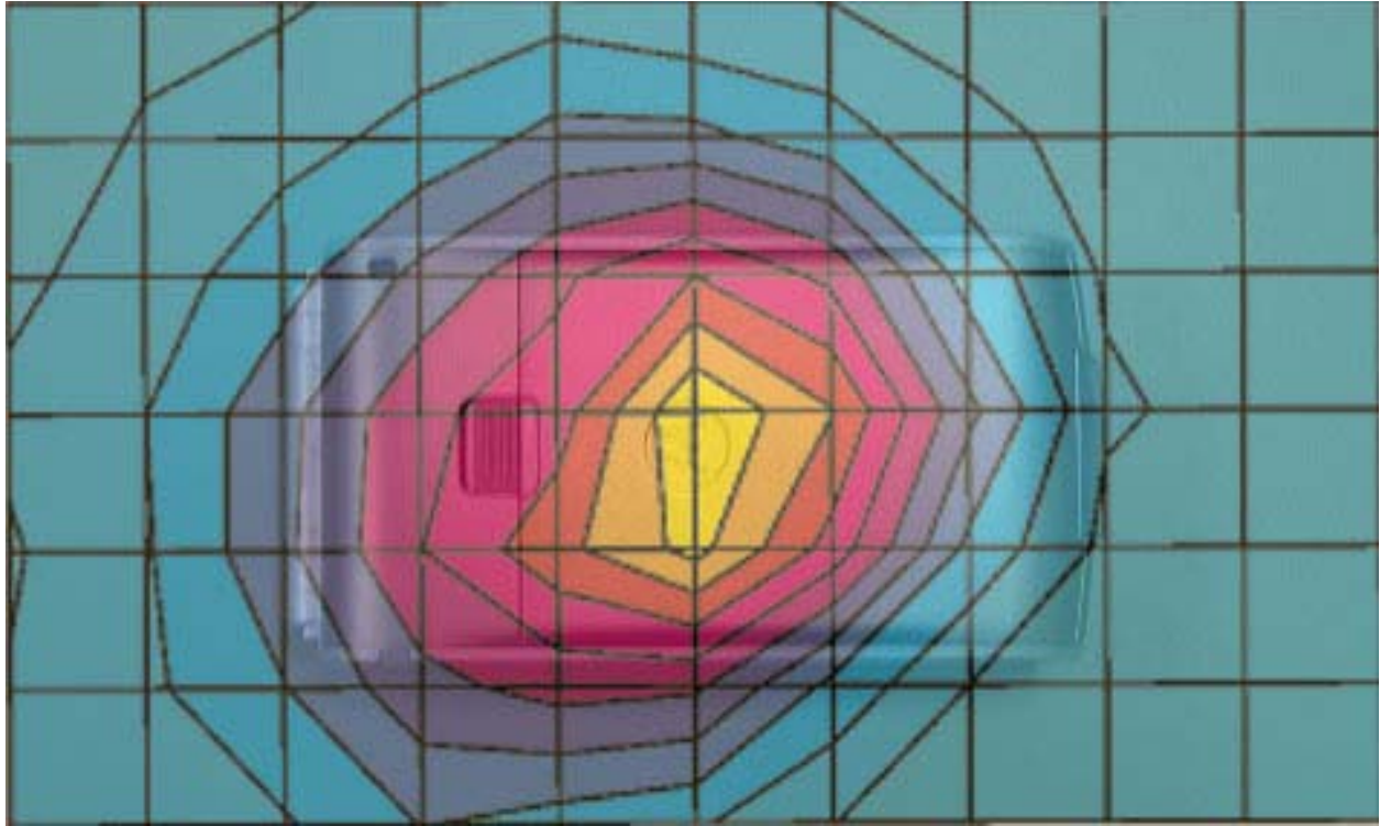
Figure 3. Typical 1900 MHz Body-Worn Contour Overlaid on Phone
