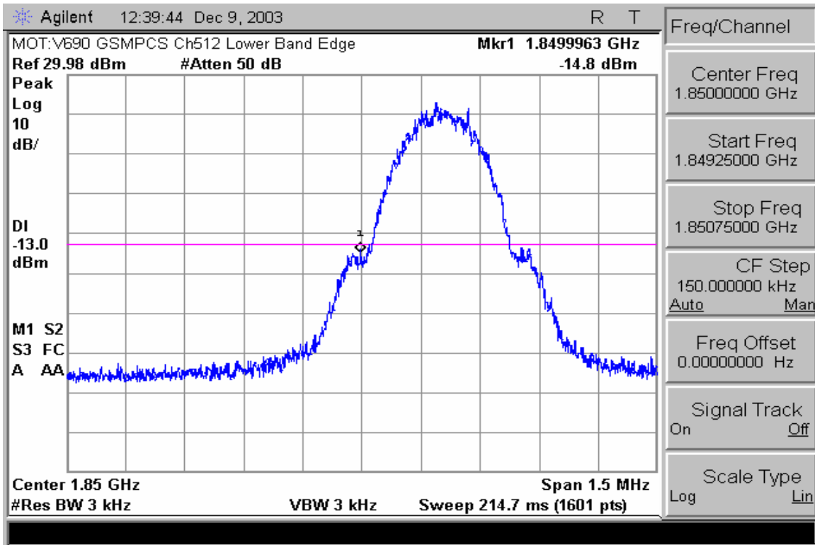
GSM/PCS 1900 Ch512 Lower Band Edge
