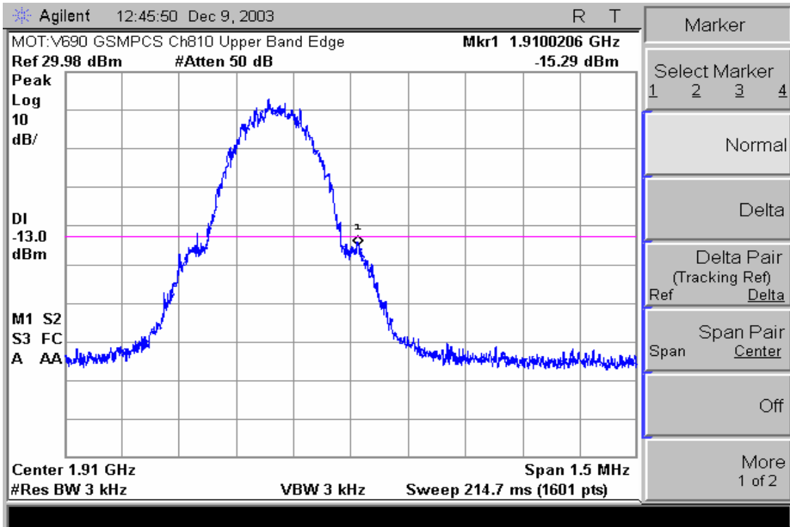
GSM/PCS 1900 Ch810 Upper Band Edge
