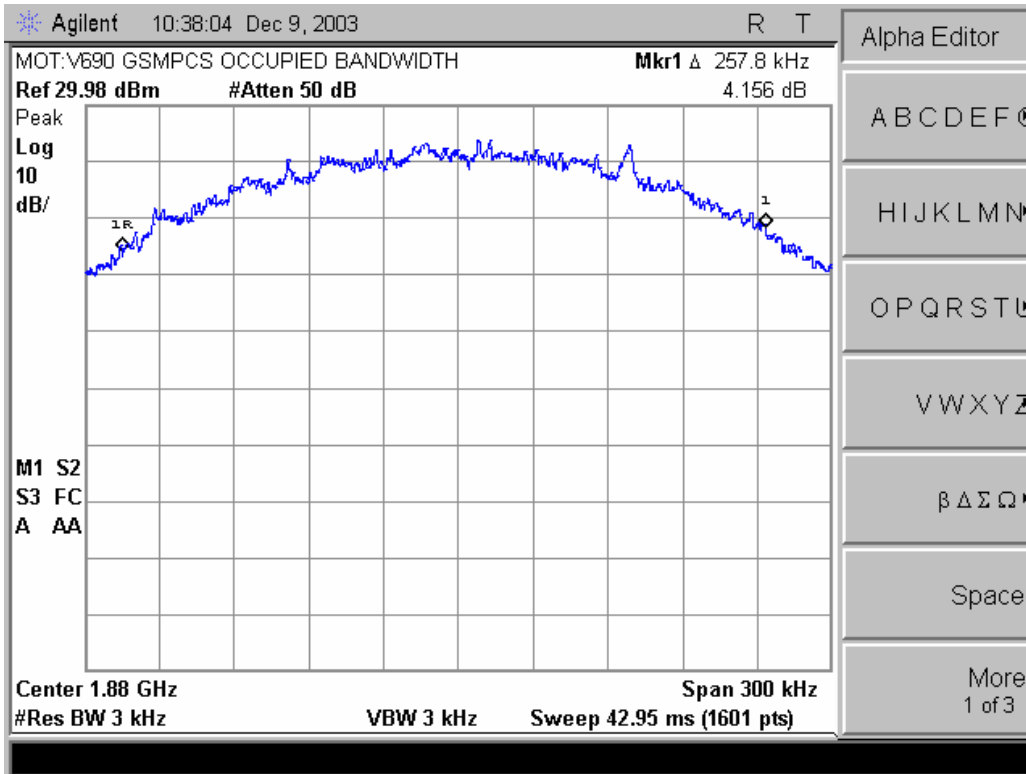
GSM/PCS 1900 Occupied Bandwidth
