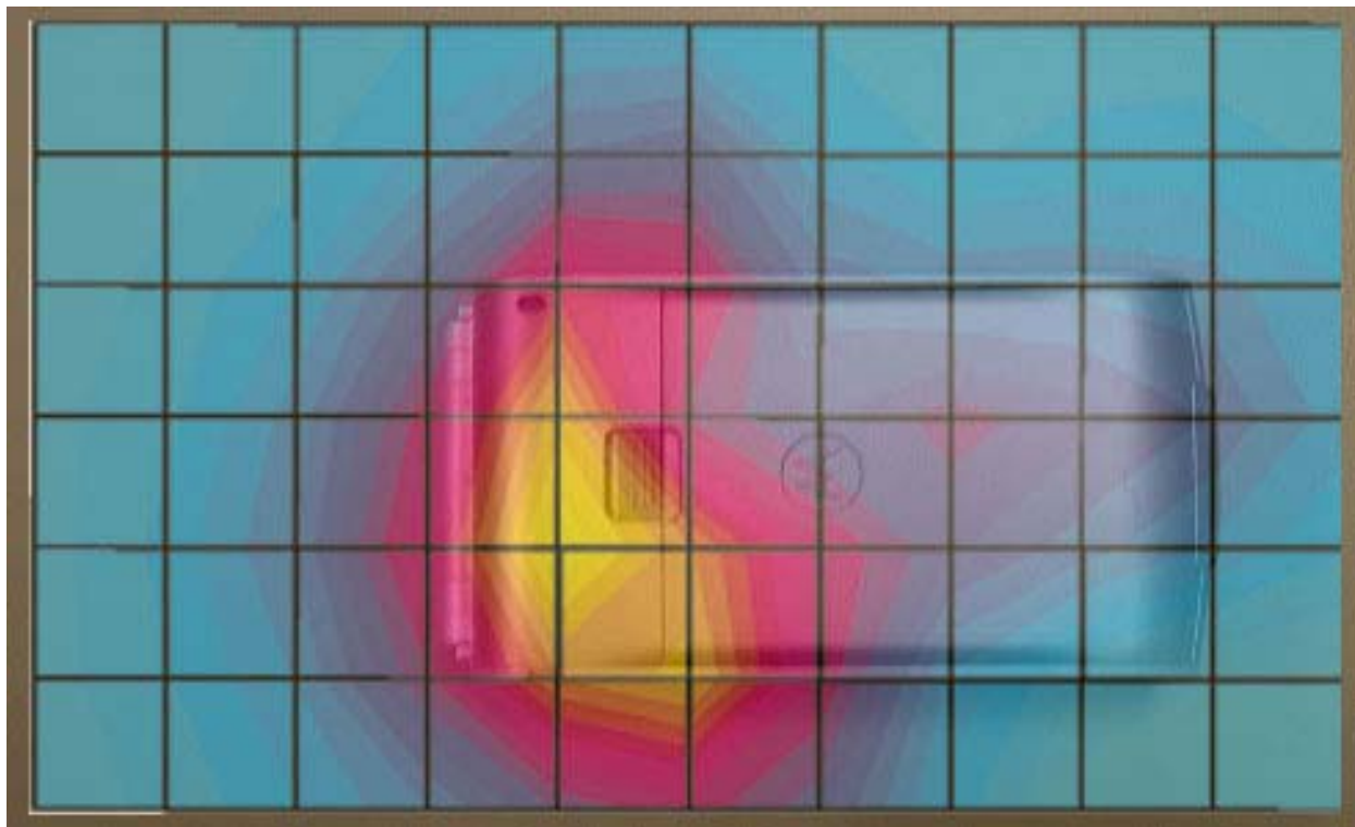
Figure 3. Typical 1900 MHz Body-Worn Contour Overlaid on Phone with Antenna Retracted
