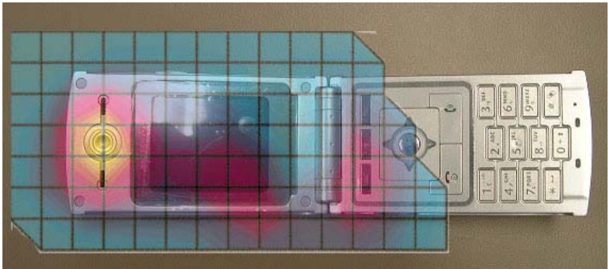
Figure 2. Typical 1900MHz Head Adjacent Contour Overlaid on Phone (15 ° Tilt)
