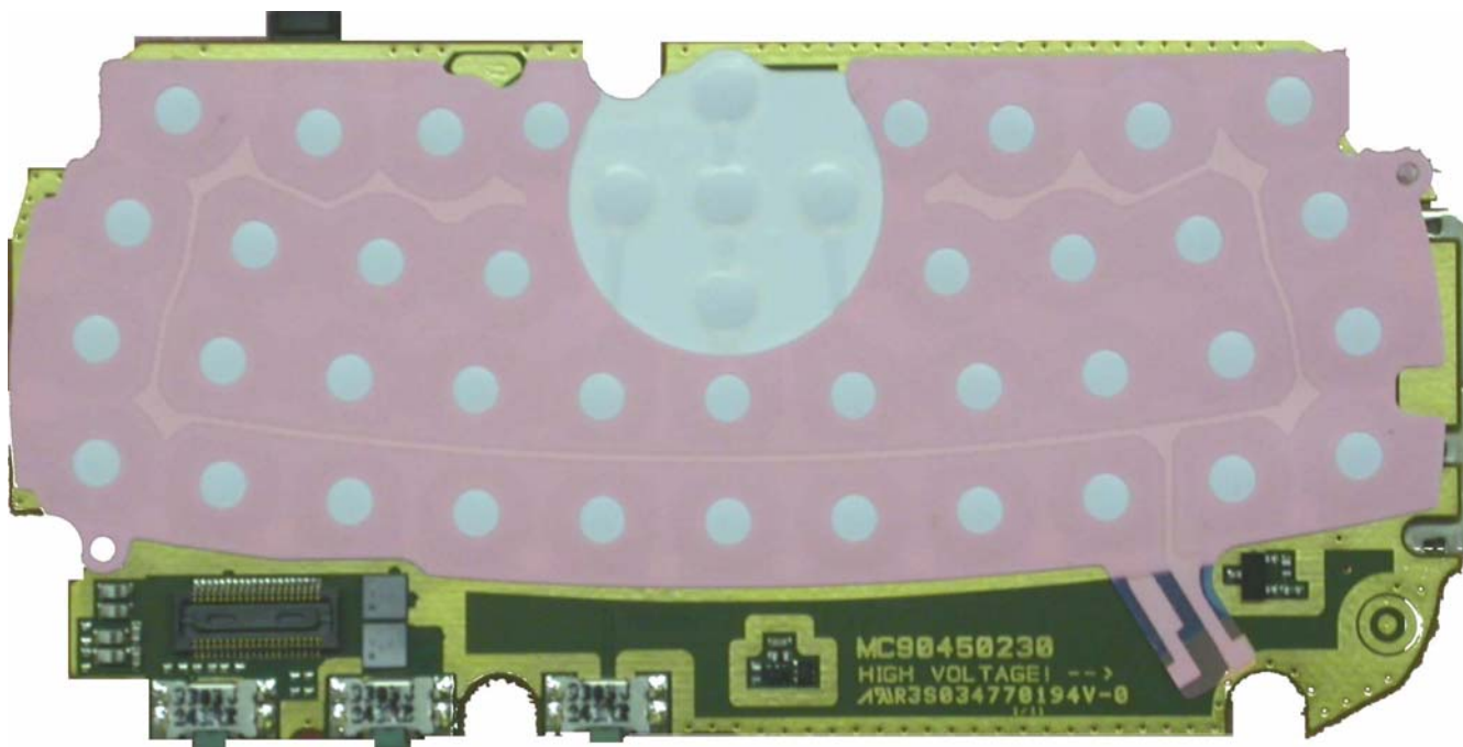
Front view (shields removed)
