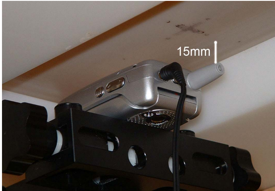
Figure 1. Back of Phone 15mm below a flat phantom
