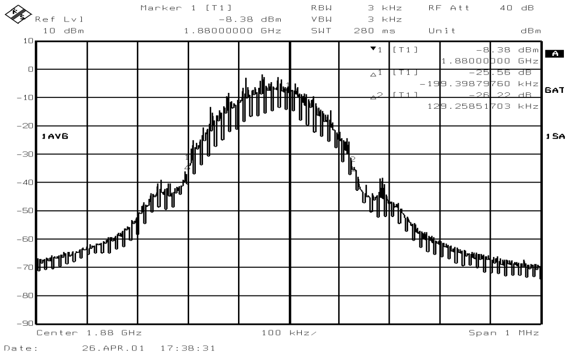
Figure 6E.3 Channel 661, 99% Power Bandwidth
