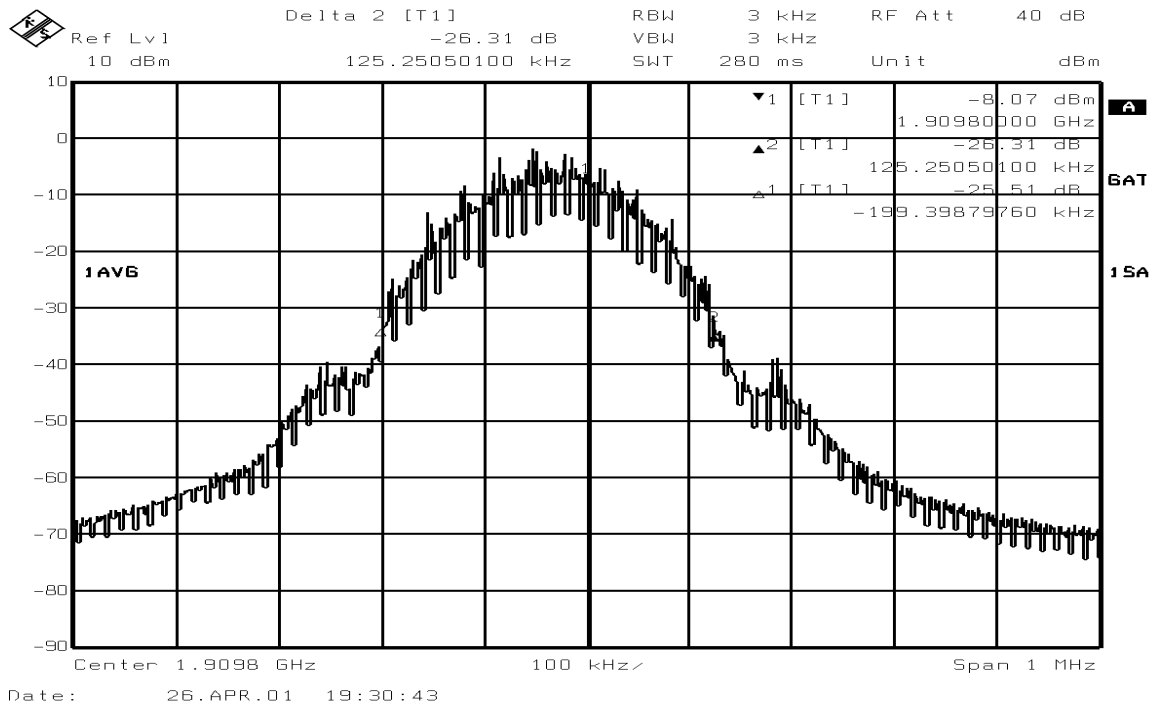
Figure 6E.6 Channel 810, -26dBc Bandwidth
