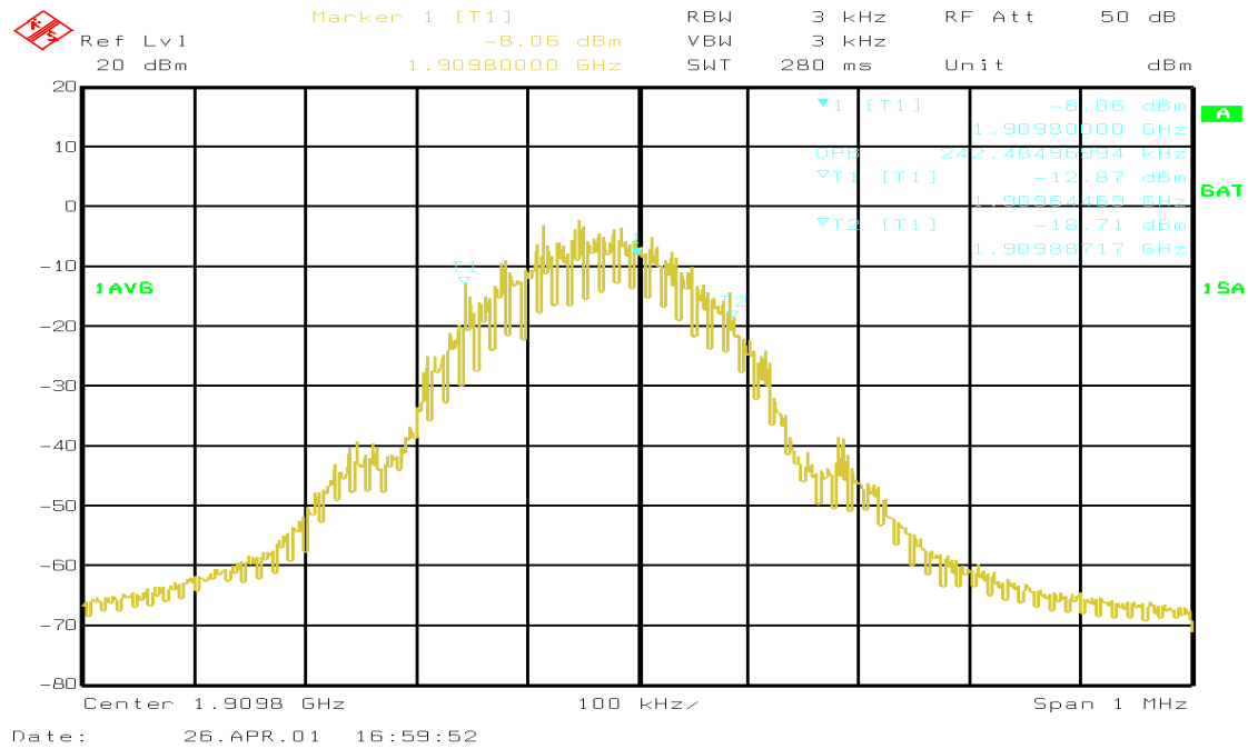
Figure 6E.5 Channel 810, 99% Power Bandwidth
