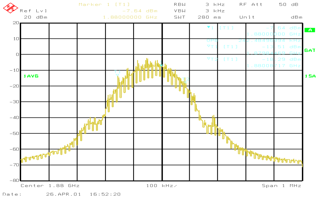
Figure 6E.3 Channel 661, 99% Power Bandwidth
