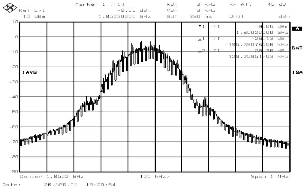
Figure 6E.2 Channel 512, -26dBc Bandwidth
