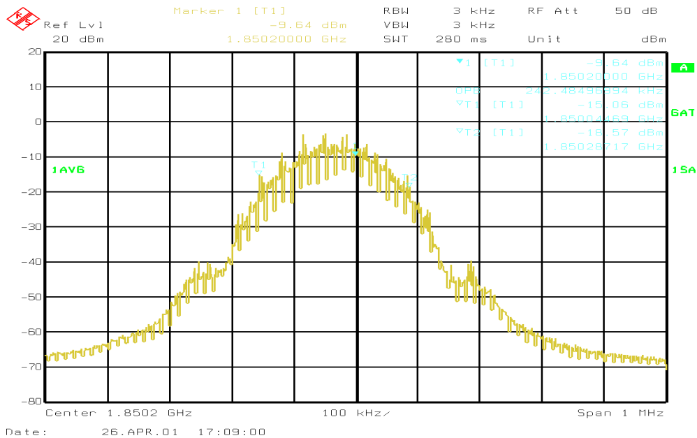
Figure 6E.1 Channel 512, 99% Power Bandwidth
