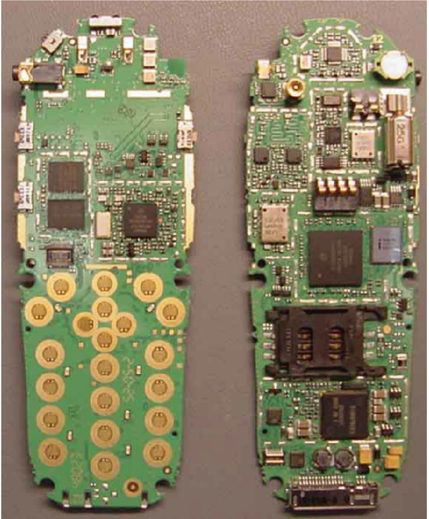
Front View (Shields Removed)
