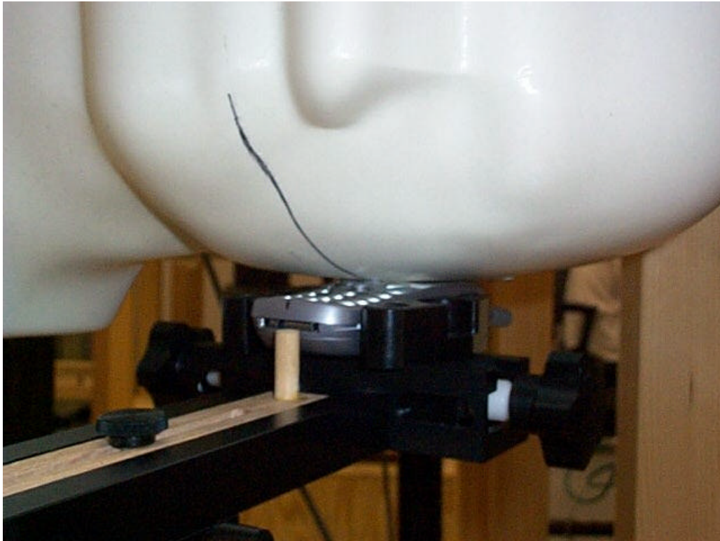
Figure 8. Phone Against the Head Phantom Front View (Cheek Touch Position)
