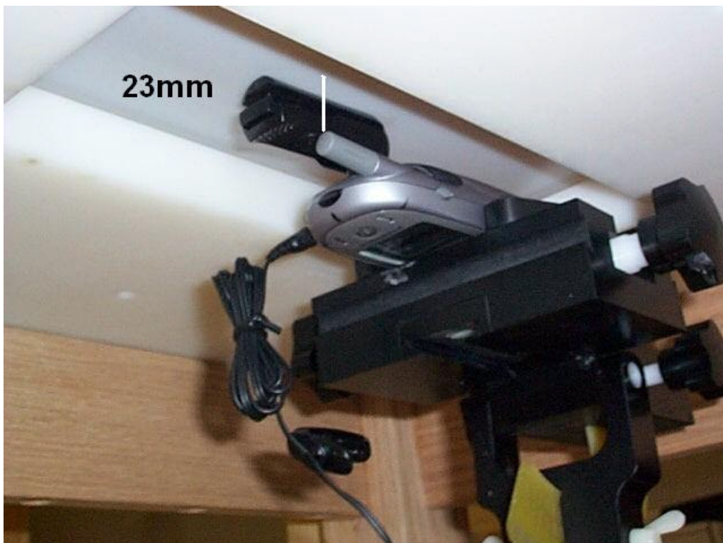
Figure 13. Phone Against the Flat Phantom with Antenna 23mm away from the base (Universal Belt Clip Attached to a Tab)
