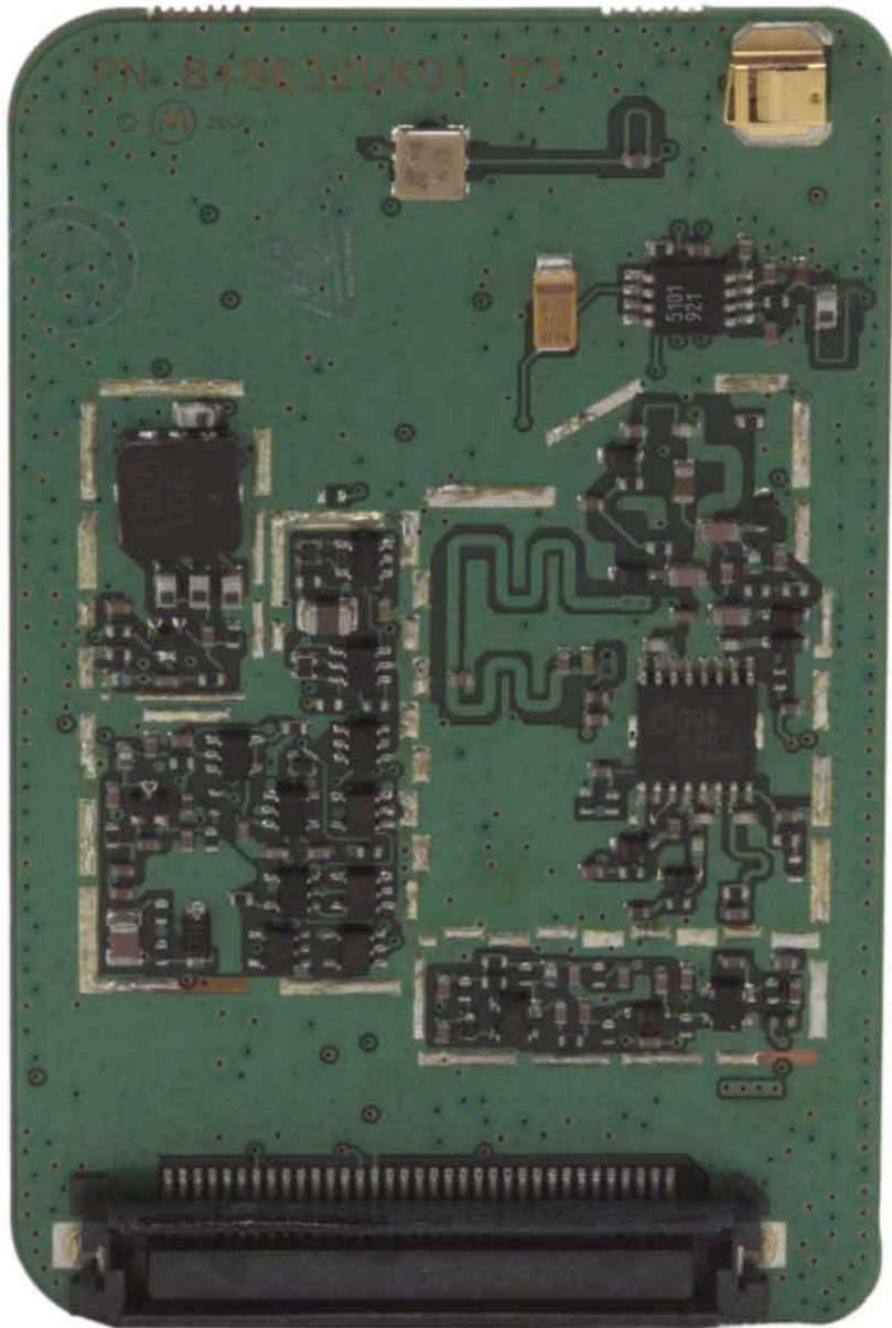
RF Board Side 1 (Shields Removed)
