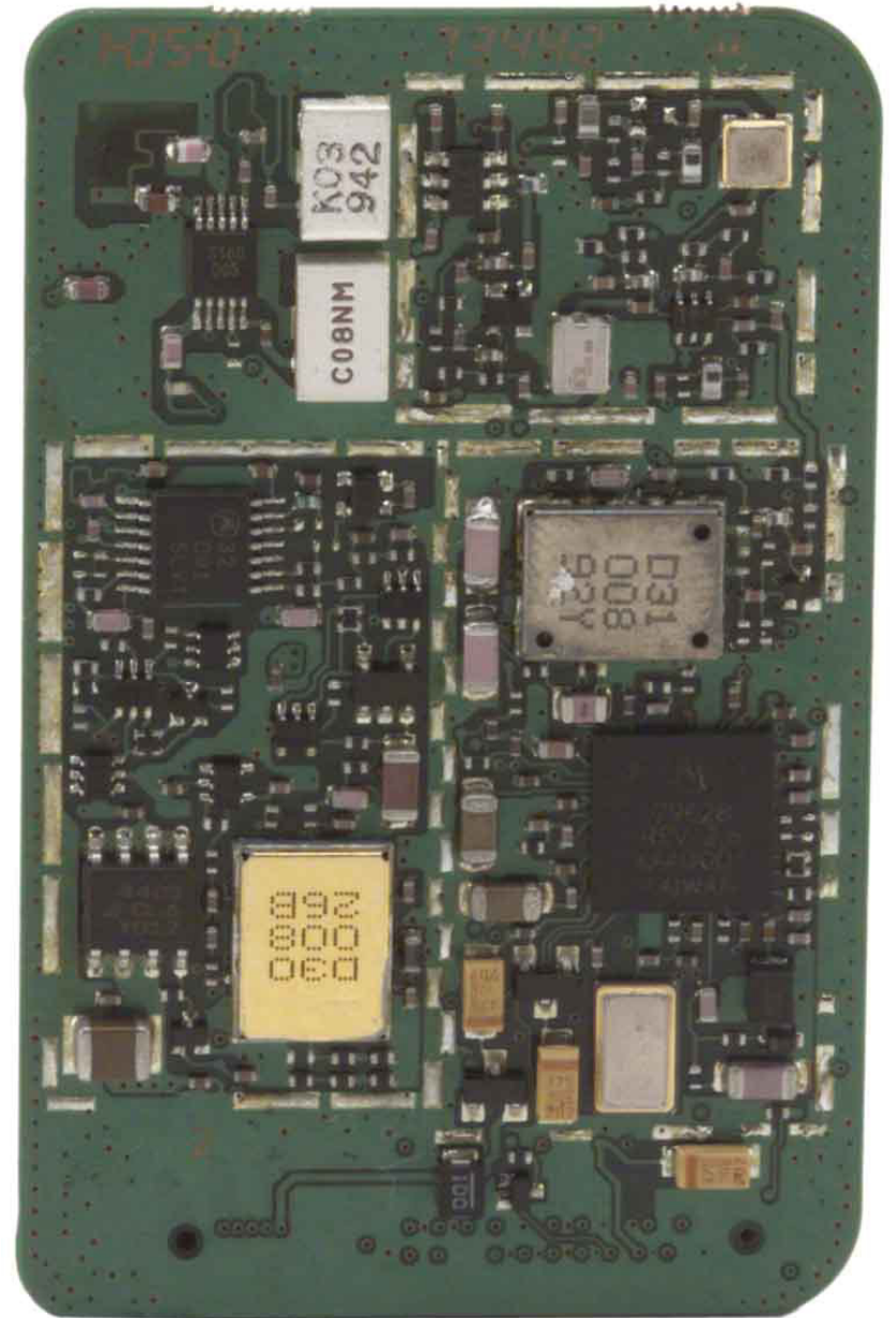
RF Board Side 2 (Shields Removed)
