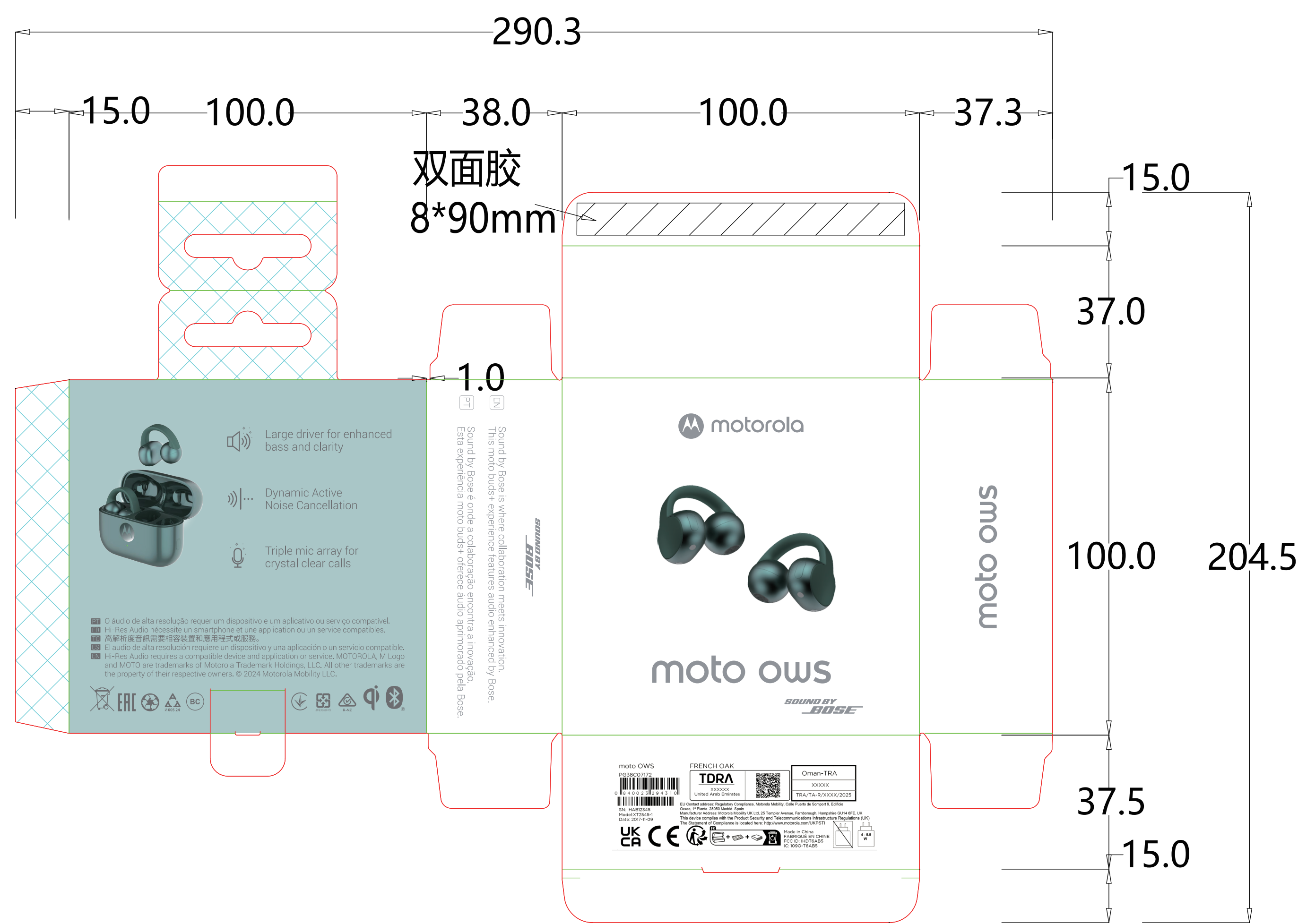
Outside box:400gC2S 纸纹
