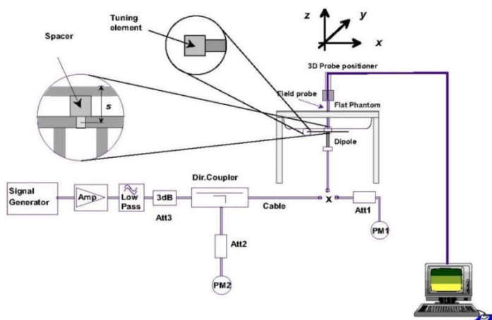
Fig 10.3.1 System Performance Check Setup
