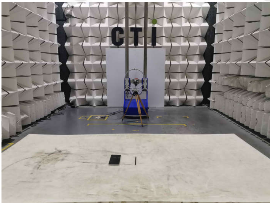
Radiated spurious emission Test Setup(9kHz~30MHz)
