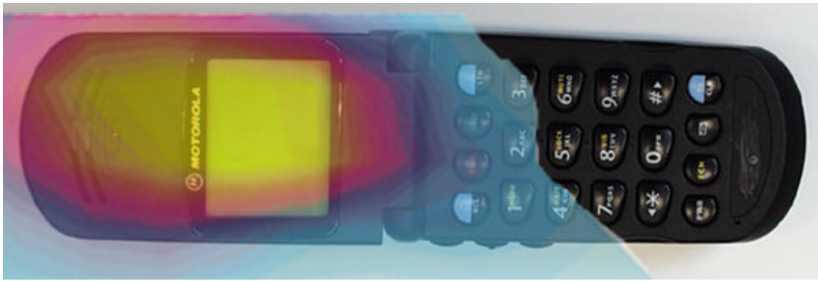
Figure 6. Digital Mode Contour Plot with Antenna Extended Overlaid on Face of Phone.
