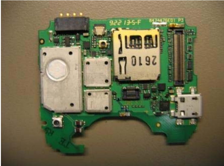
Main Board Back with Shields
