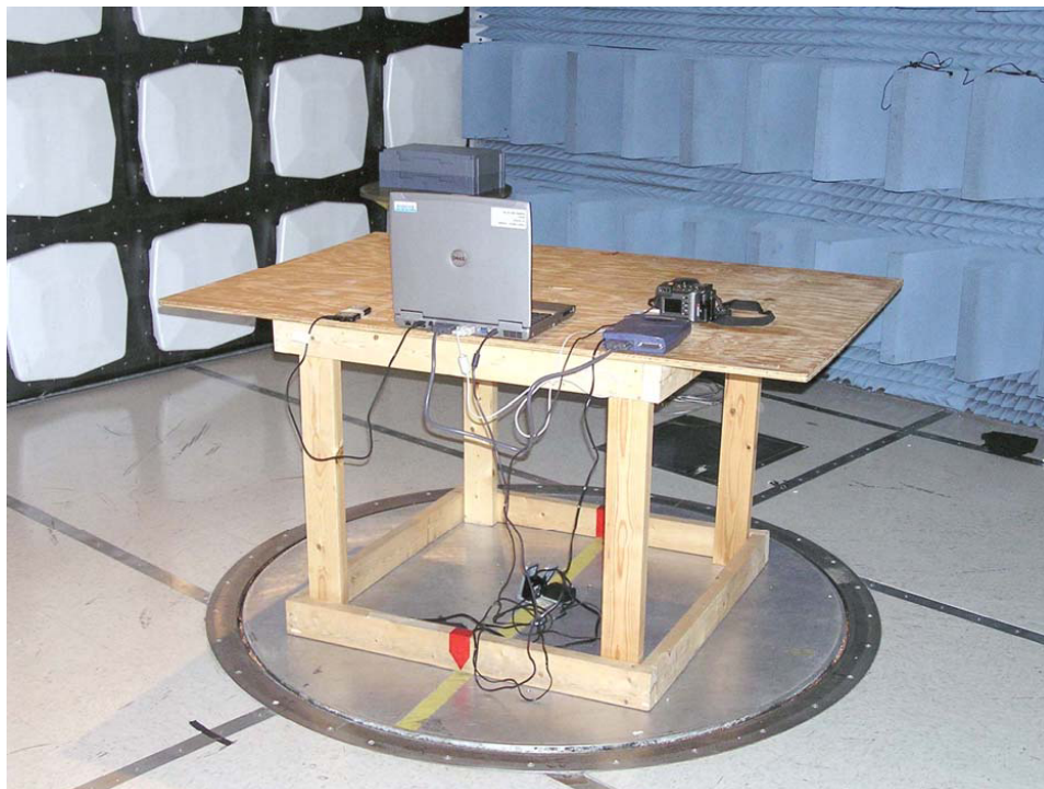
Computer Peripheral Radiated Emissions Measurement Setup
