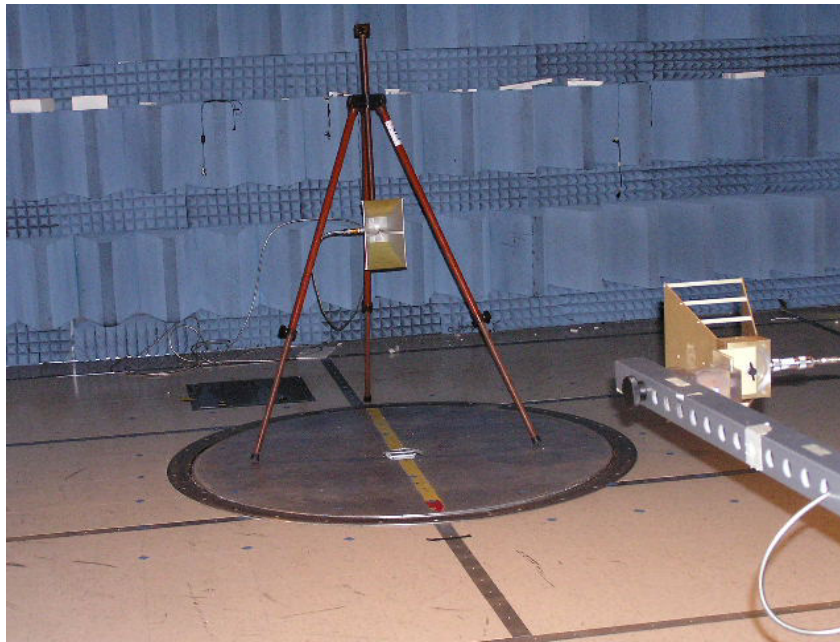
Antenna Substitution Measurement
