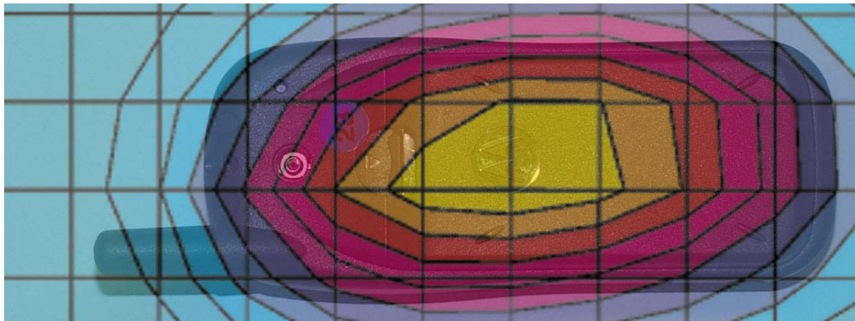
Figure 5. Typical AMPS Body-Worn Contour Overlaid on Phone
