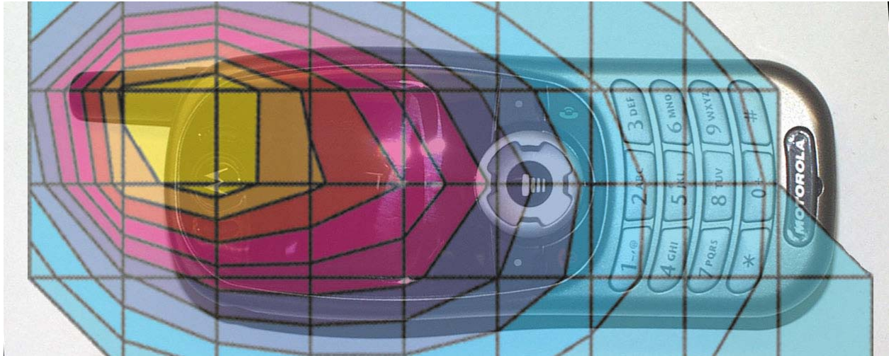
Figure 3. Typical AMPS Head Adjacent Contour Overlaid on Phone (15 ° Tilt)
