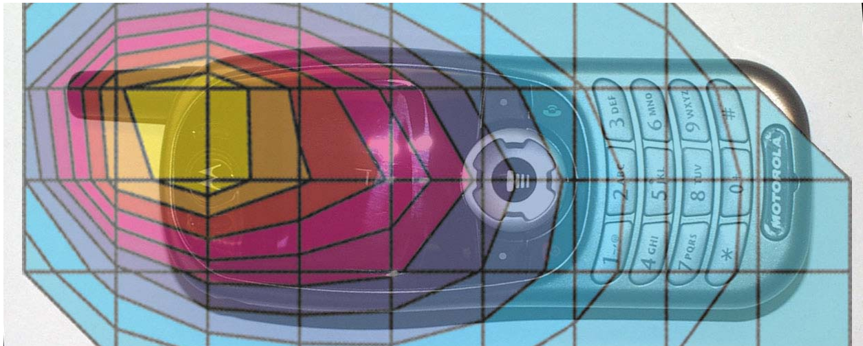
Figure 4. Typical CDMA Head Adjacent Contour Overlaid on Phone (15 ° Tilt)
