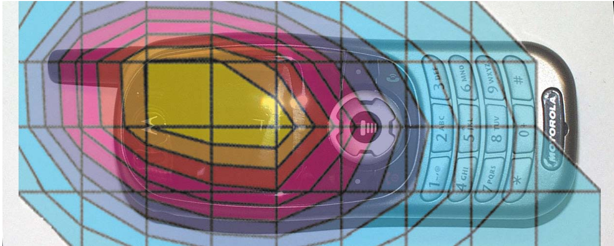
Figure 1. Typical AMPS Head Adjacent Contour Overlaid on Phone (Cheek Touch)
