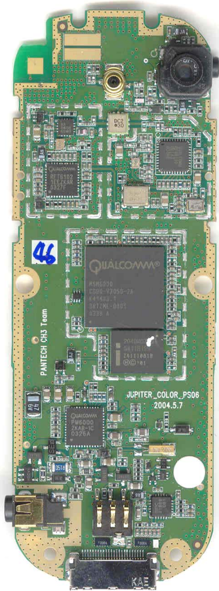
Rear View (without shields)
