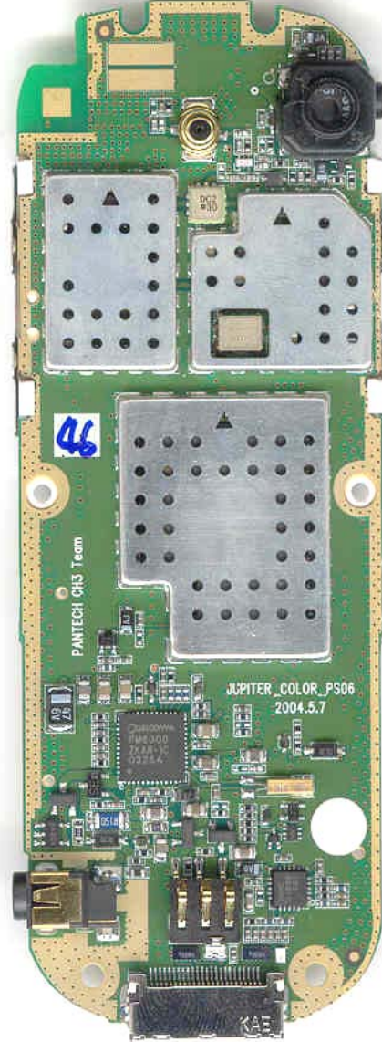
Rear View
