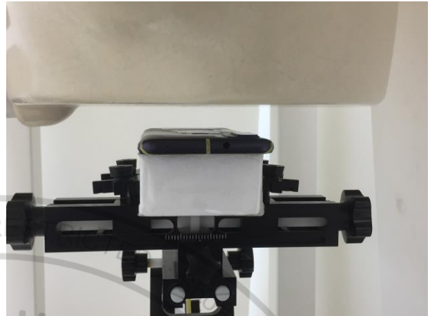
Back, Test Separation 24 mm
