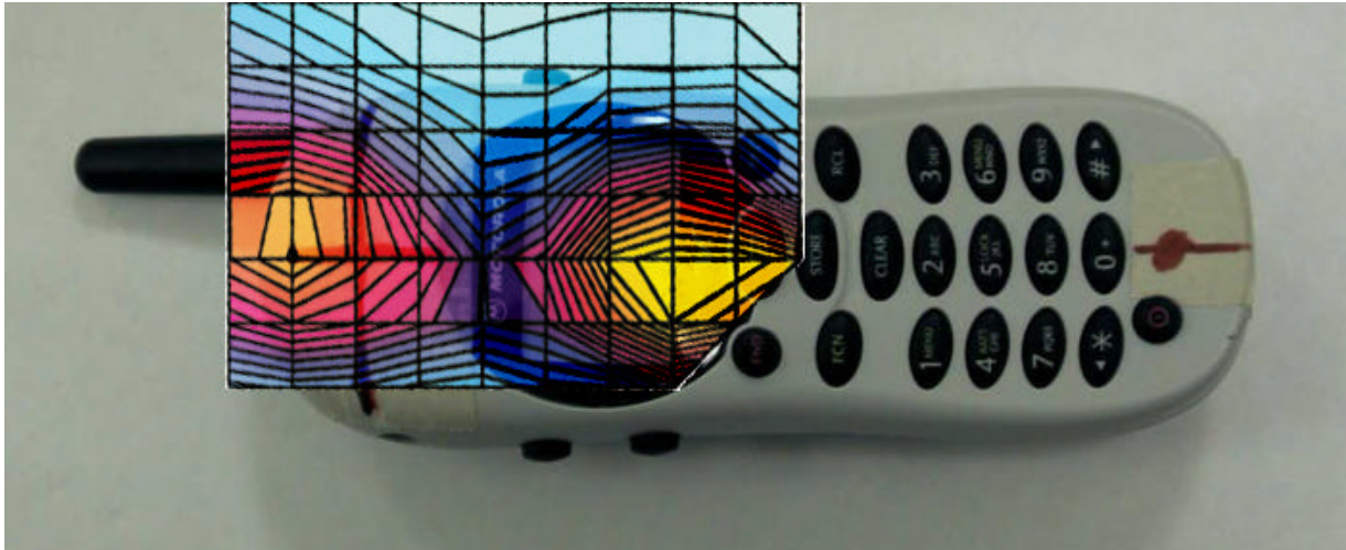
Figure 5. 1900MHz Contour Plot Overlaid on Face of Phone.
