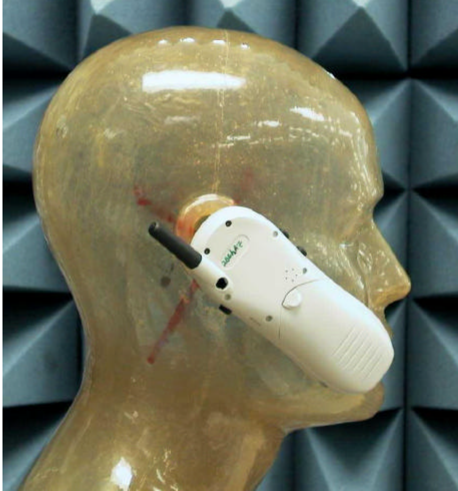
Figure 2. Phone against side of Phantom Head.
