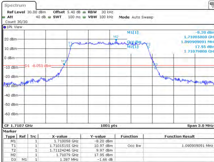
Band66-1.4MHz-QPSK-131979-6RB#0-1.091
