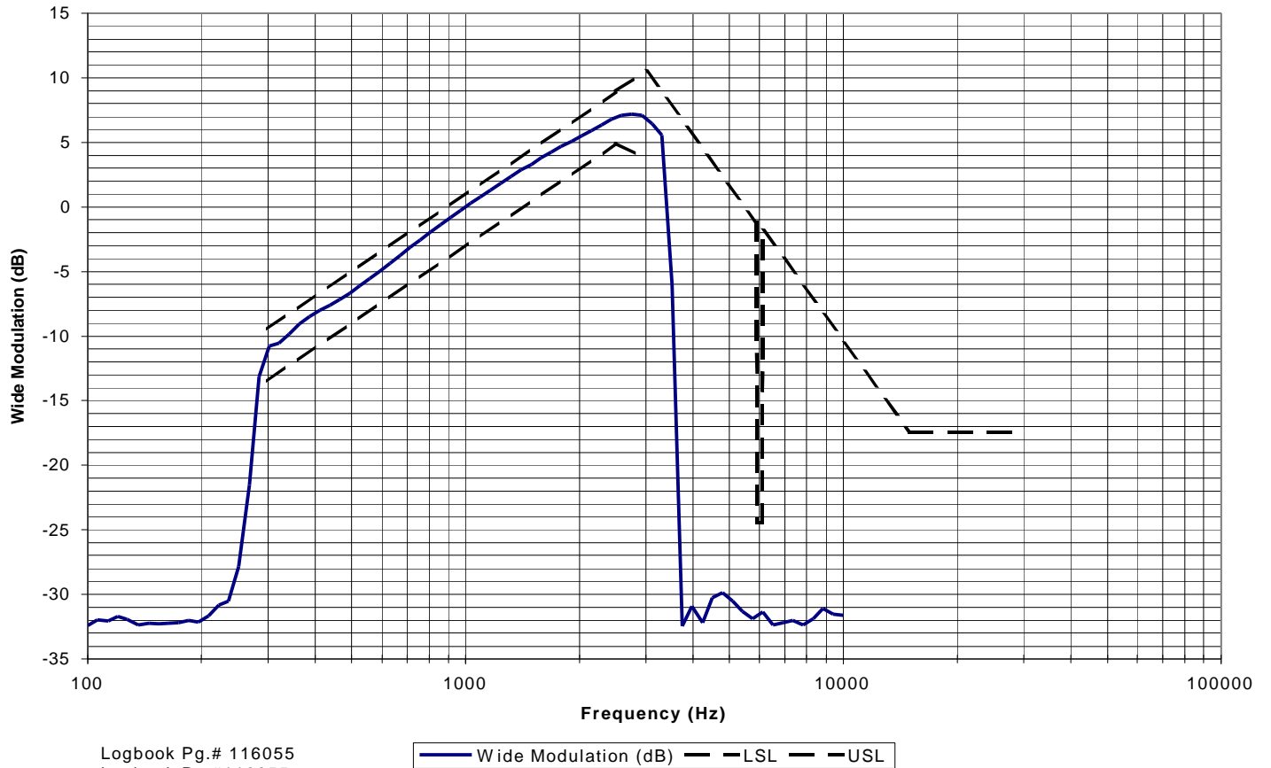
Tx Audio Response -- Wide Mode
