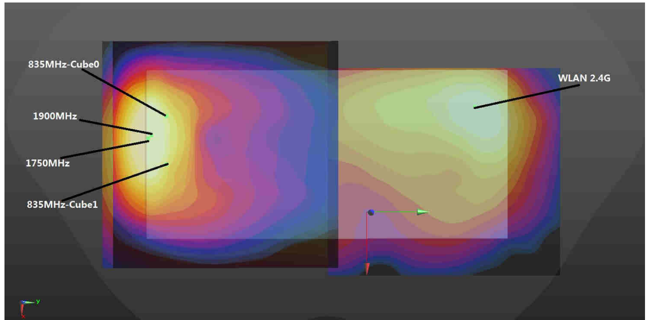
WWAN(5mm)+2.4GHz(5mm)
