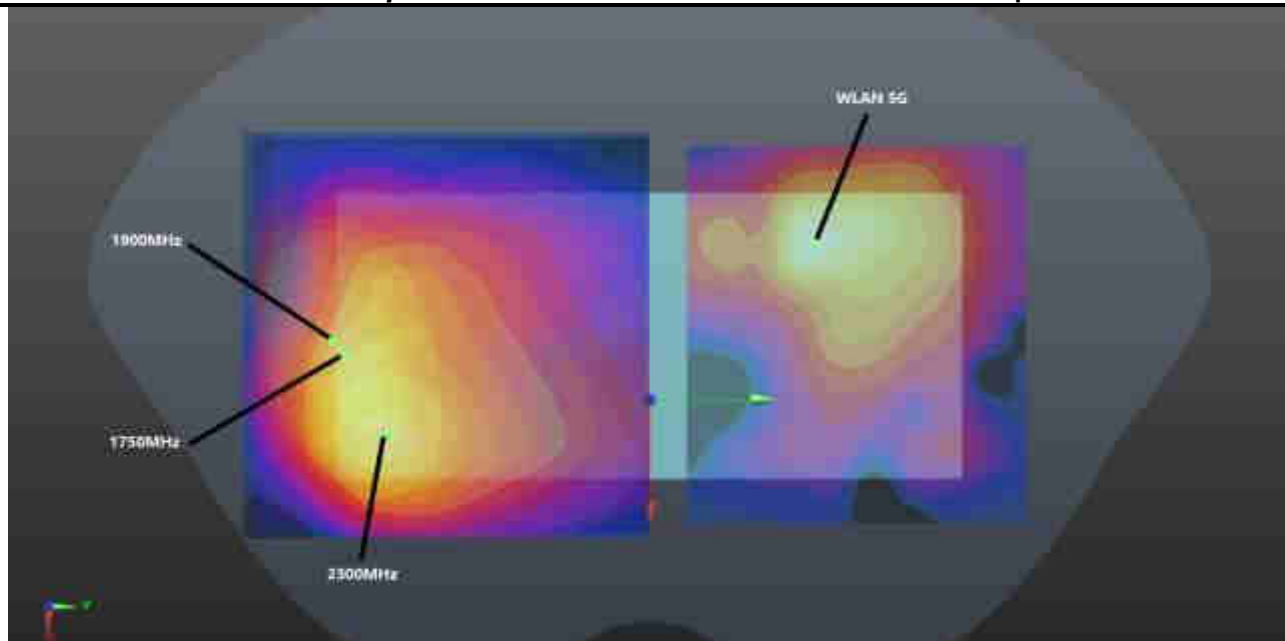
WWAN (0mm)+5G(0mm) Back
