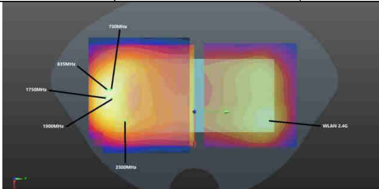
WWAN (5mm)+2.4G(5mm) Front
