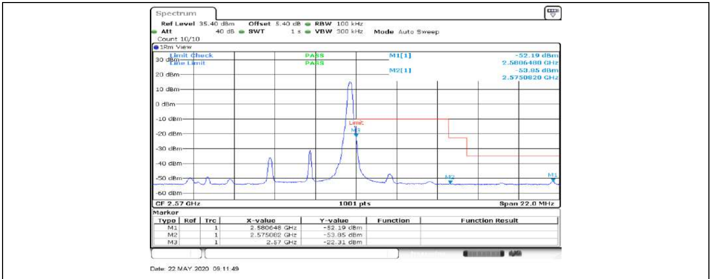
Band7-5MHz-64QAM-21425-25RB#0
