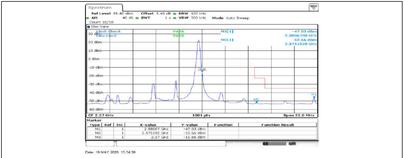
Band7-5MHz-16QAM-21425-25RB#0
