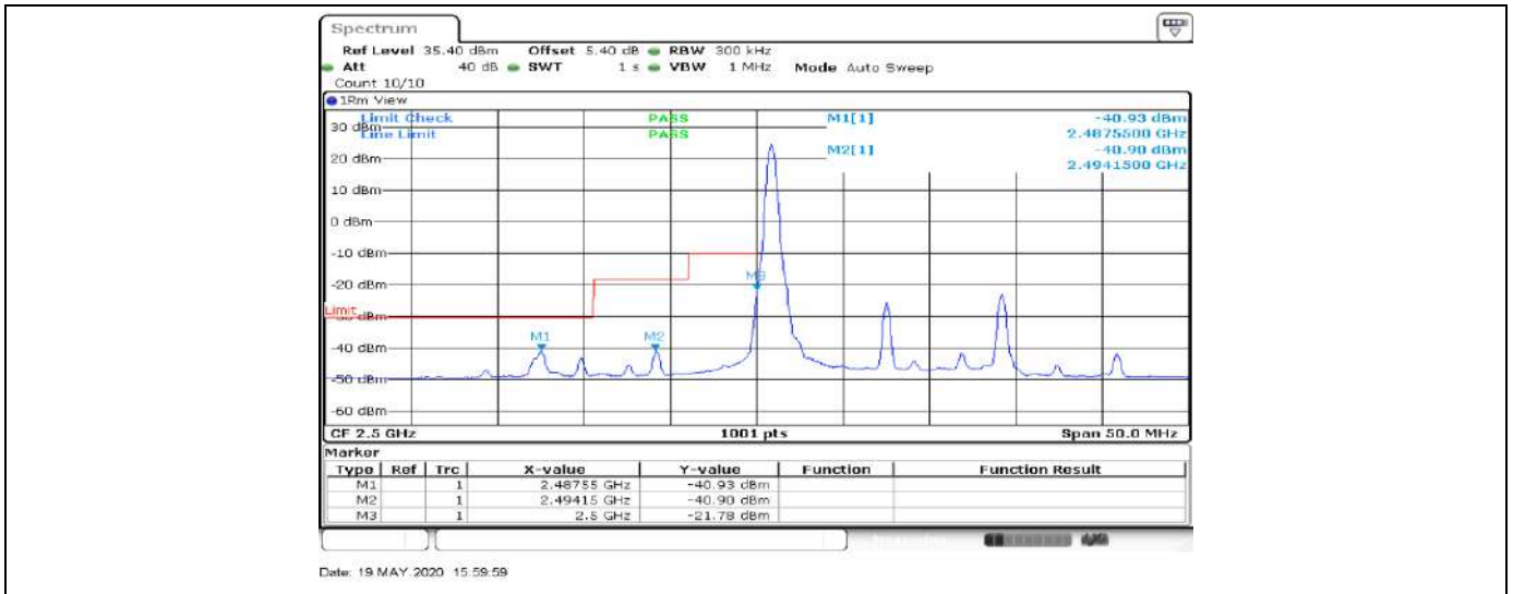
Band7-15MHz-16QAM-20825-75RB#0
