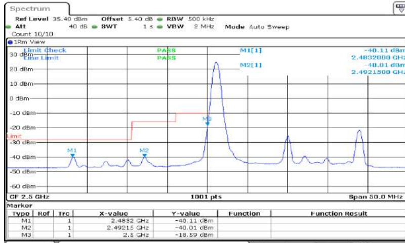
Band7-20MHz-16QAM-20850-100RB#0
