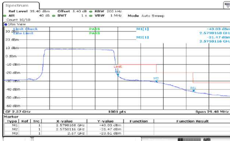
Band7-10MHz-QPSK-21400-50RB#0
