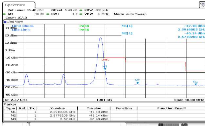
Band7-20MHz-64QAM-21350-100RB#0
