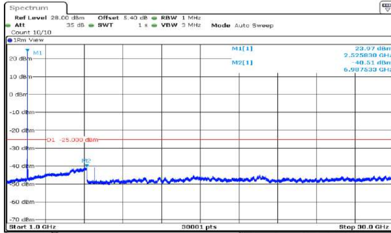
Band7-20MHz-16QAM-21100-1RB#0-Range2:1000~30000MHz
