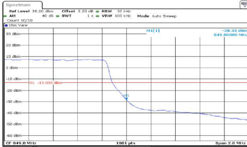
Band5-1.4MHz-16QAM-20643-6RB#0
