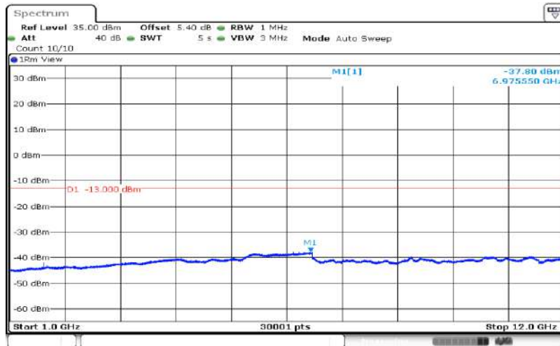
Band5-10MHz-16QAM-20525-1RB#0-Range2:1000~12000MHz
