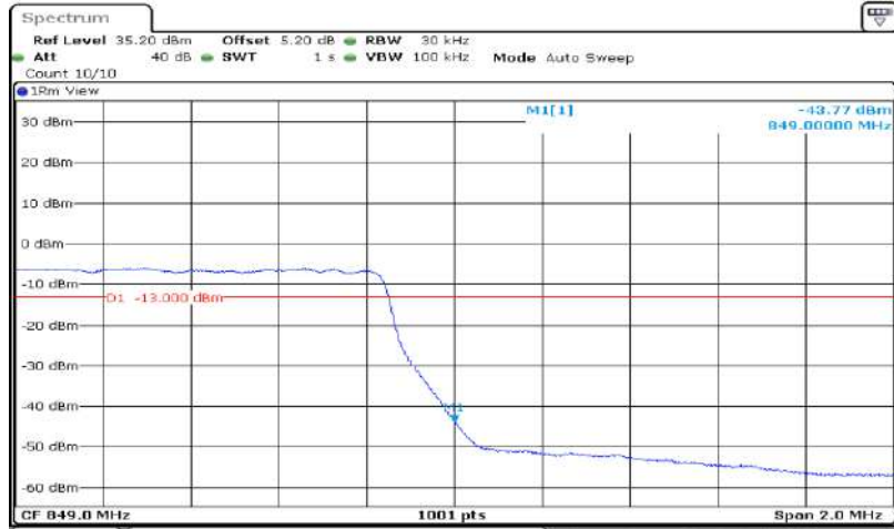
Band5-1.4MHz-64QAM-20643-6RB#0
