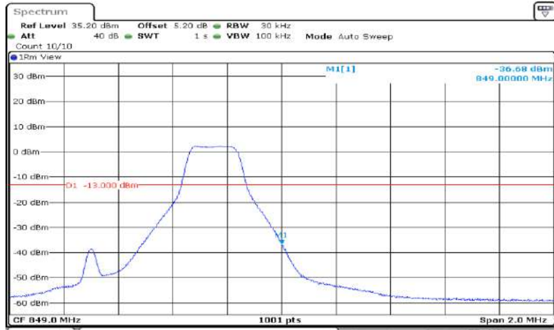
Band5-1.4MHz-64QAM-20643-6RB#0
