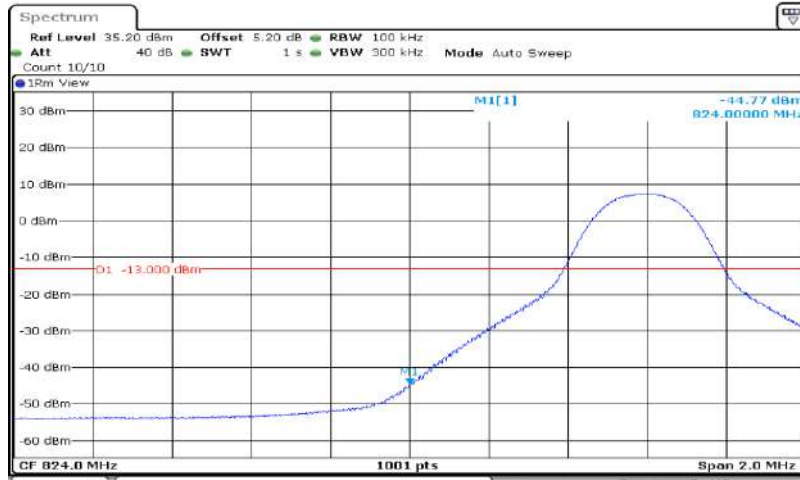
Band5-10MHz-64QAM-20450-50RB#0
