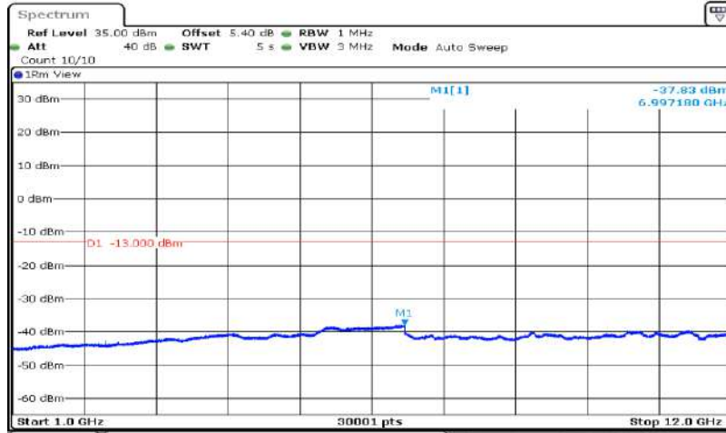
Band5-10MHz-64QAM-20600-1RB#0-Range2:1000~12000MHz
