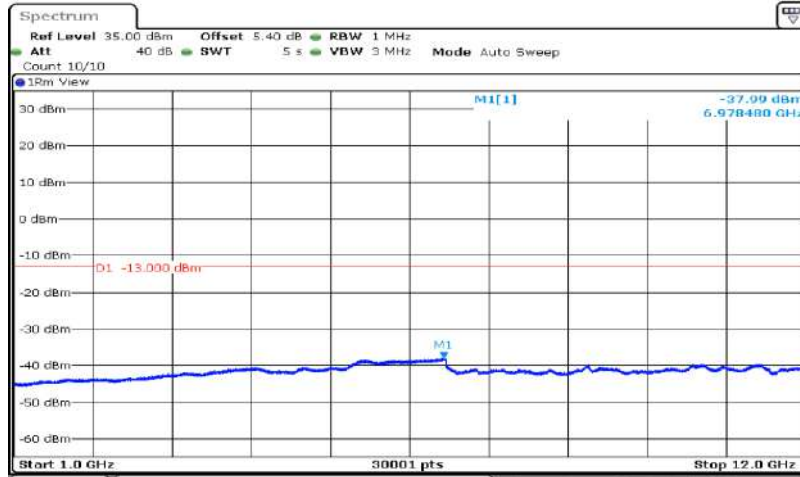
Band5-10MHz-64QAM-20450-1RB#0-Range2:1000~12000MHz
