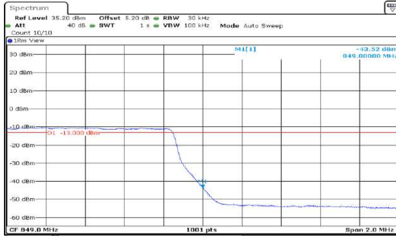
Band5-3MHz-64QAM-20635-15RB#0
