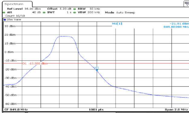
Band5-5MHz-16QAM-20625-25RB#0
