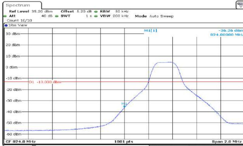
Band5-5MHz-64QAM-20425-25RB#0
