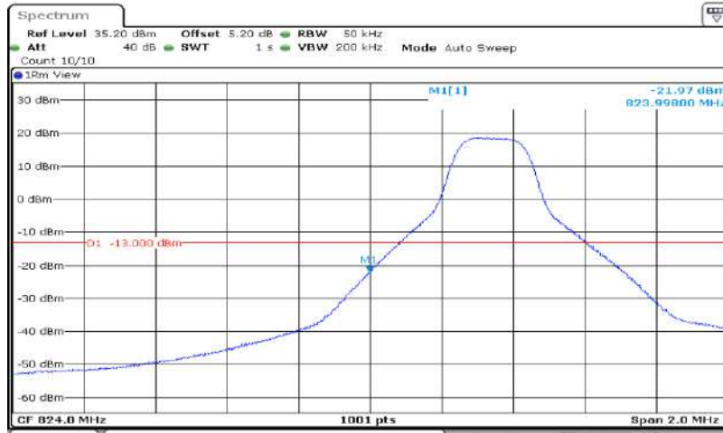
Band5-5MHz-16QAM-20425-25RB#0
