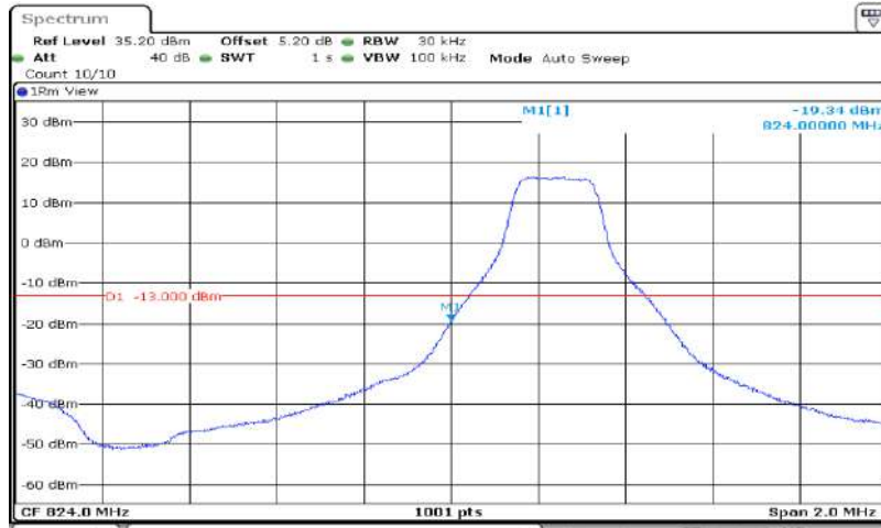
Band5-3MHz-16QAM-20415-15RB#0
