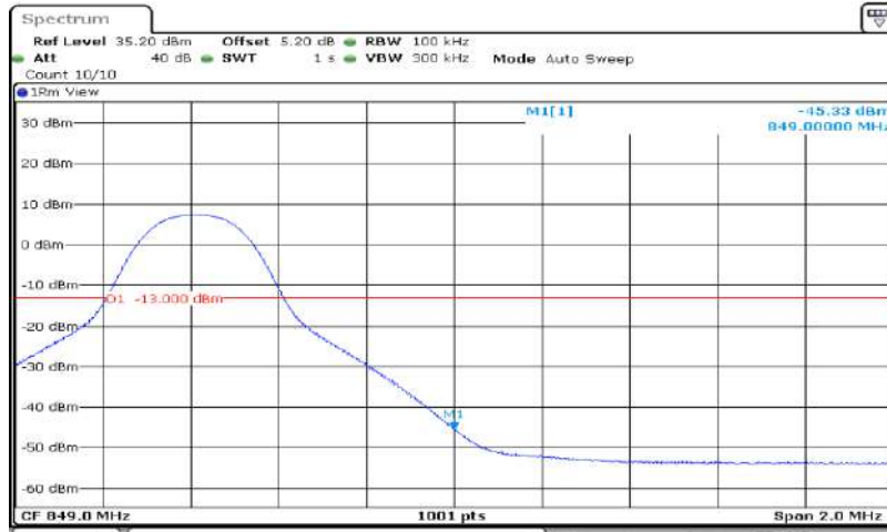
Band5-10MHz-64QAM-20600-50RB#0
