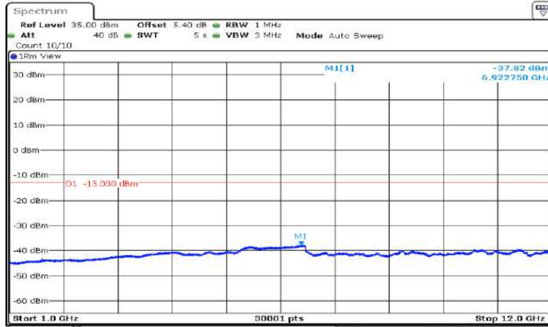
Band5-10MHz-16QAM-20450-1RB#0-Range2:1000~12000MHz
