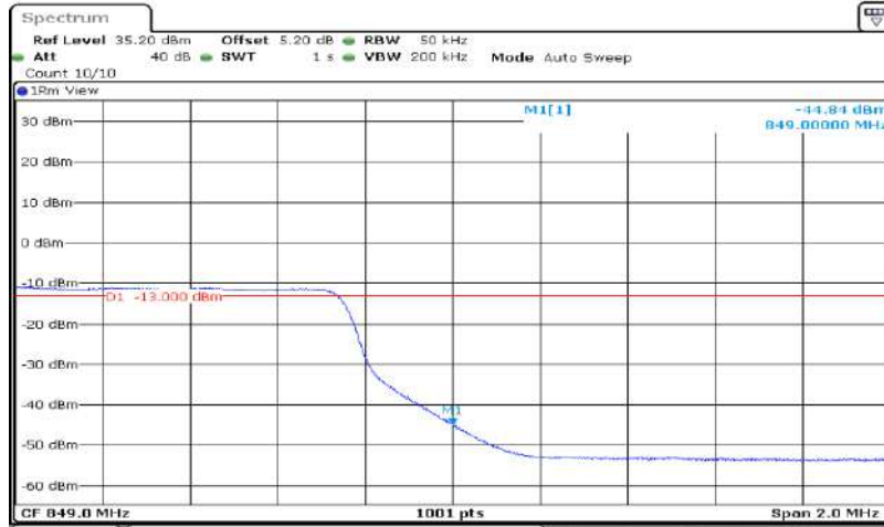
Band5-5MHz-64QAM-20625-25RB#0
