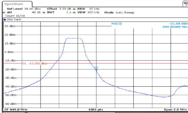
Band5-3MHz-16QAM-20635-15RB#0
