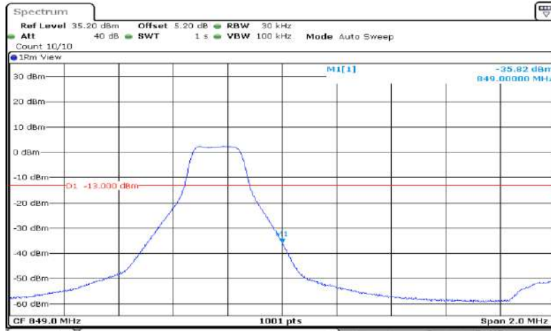
Band5-3MHz-64QAM-20635-15RB#0
