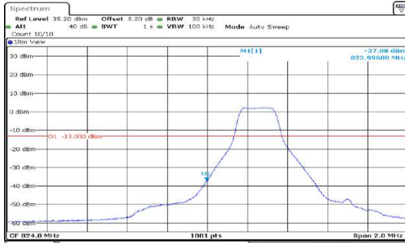
Band5-1.4MHz-64QAM-20407-6RB#0
