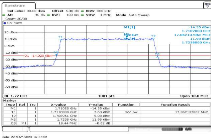
Band4-20MHz-QPSK-20175-100RB#0-17.862
