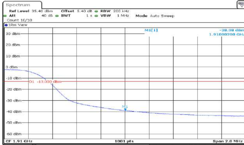
Band2-15MHz-16QAM-19125-75RB#0
