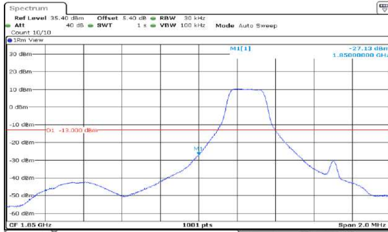
Band2-1.4MHz-16QAM-18607-6RB#0
