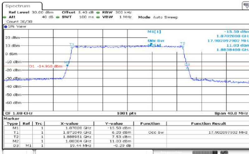
Band2-20MHz-QPSK-19100-100RB#0-17.902
