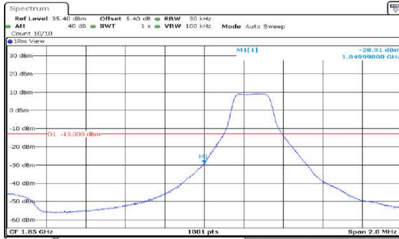
Band2-3MHz-64QAM-18615-15RB#0
