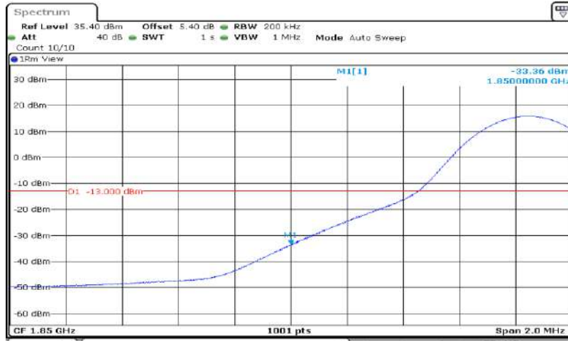
Band2-15MHz-64QAM-18675-75RB#0
