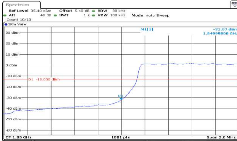
Band2-1.4MHz-16QAM-18607-6RB#0
