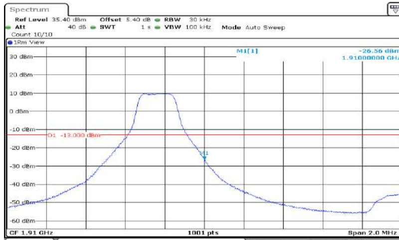
Band2-3MHz-64QAM-19185-15RB#0
