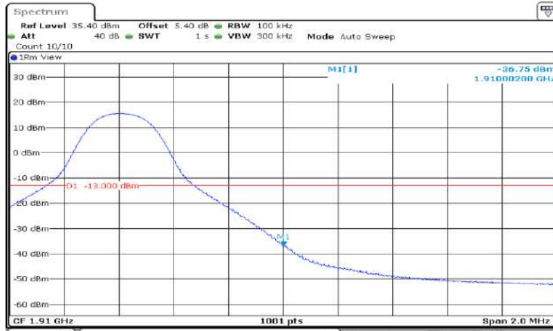
Band2-10MHz-16QAM-19150-50RB#0
