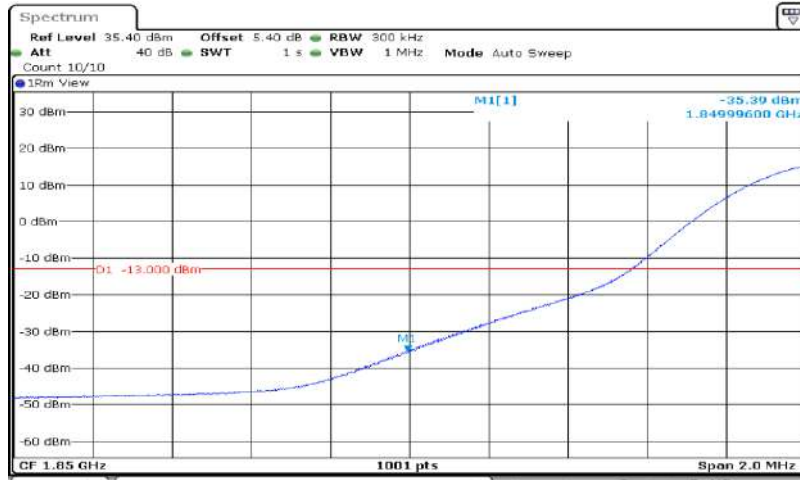
Band2-20MHz-64QAM-18700-100RB#0
