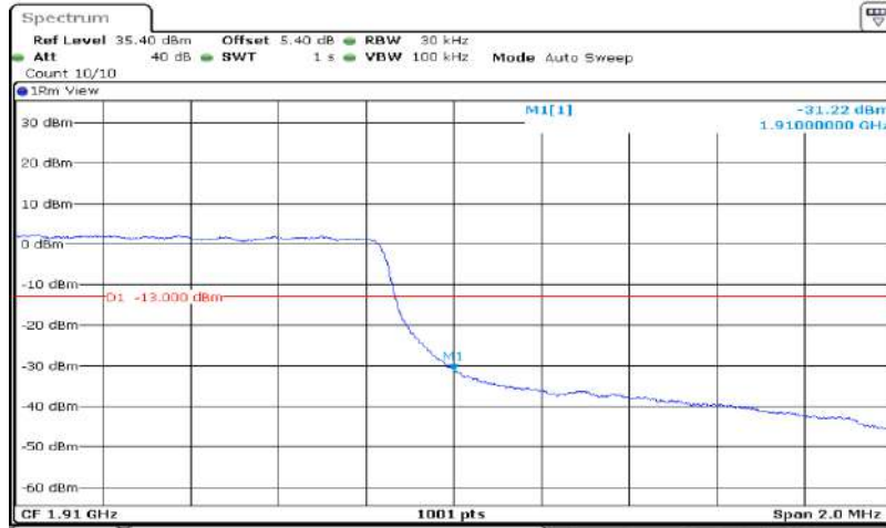
Band2-1.4MHz-16QAM-19193-6RB#0
