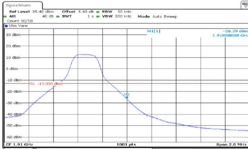
Band2-5MHz-16QAM-19175-25RB#0
