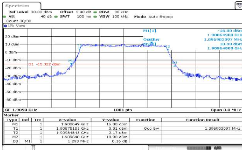
Band2-1.4MHz-64QAM-19193-6RB#0-1.097
