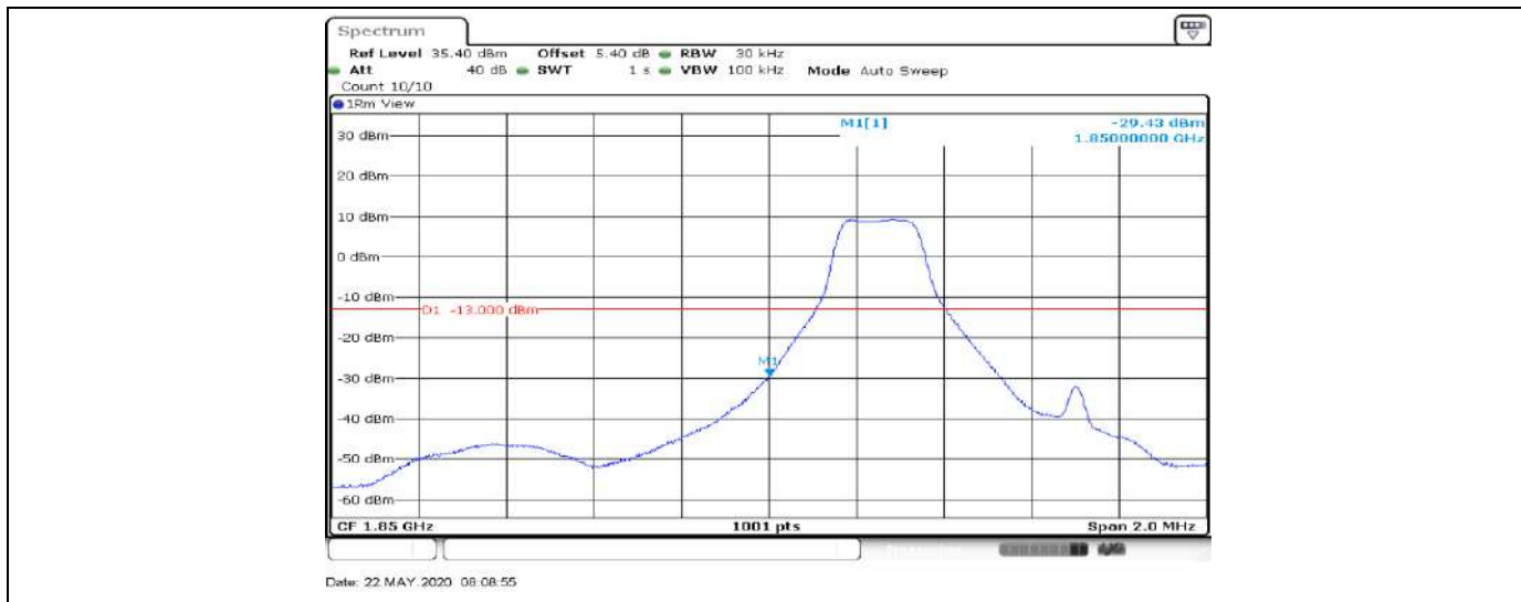
Band2-1.4MHz-64QAM-18607-6RB#0
