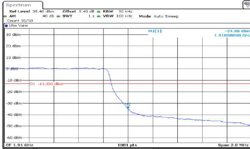
Band2-1.4MHz-64QAM-19193-6RB#0
