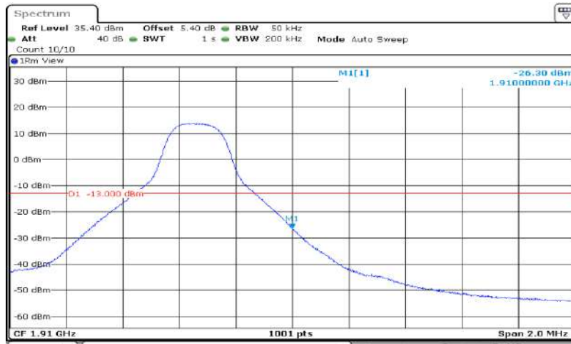
Band2-5MHz-QPSK-19175-25RB#0
