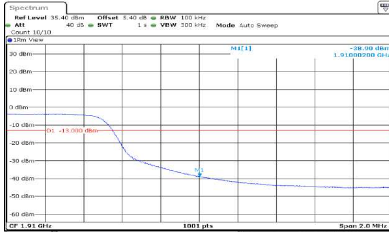
Band2-10MHz-16QAM-19150-50RB#0
