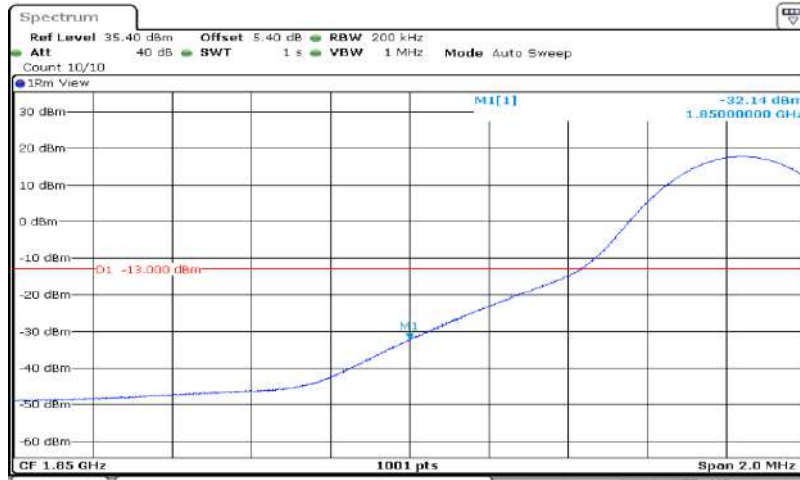
Band2-15MHz-QPSK-18675-75RB#0
