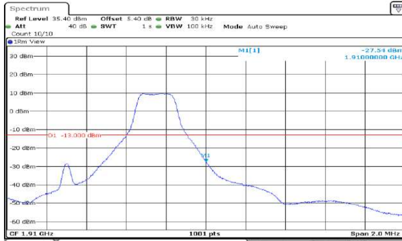
Band2-1.4MHz-64QAM-19193-6RB#0
