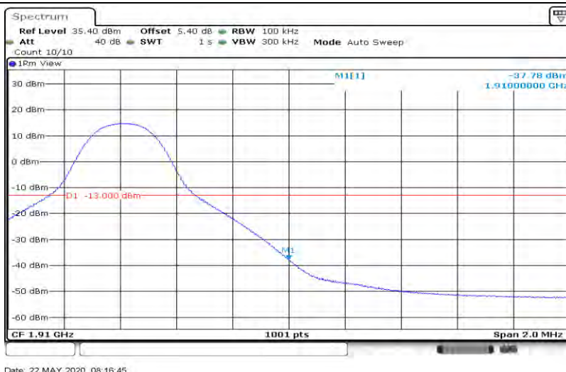
Band2-10MHz-64QAM-19150-50RB#0
