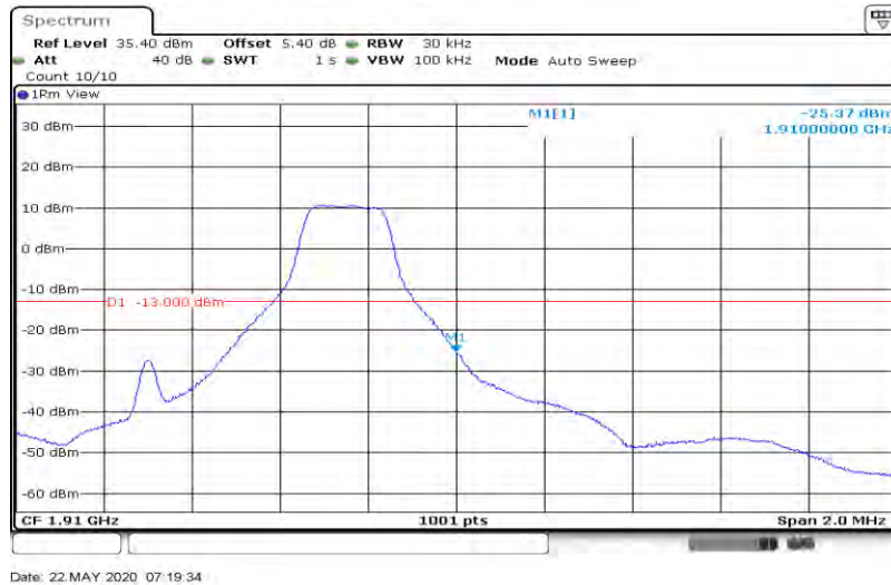
Band2-1.4MHz-16QAM-19193-6RB#0
