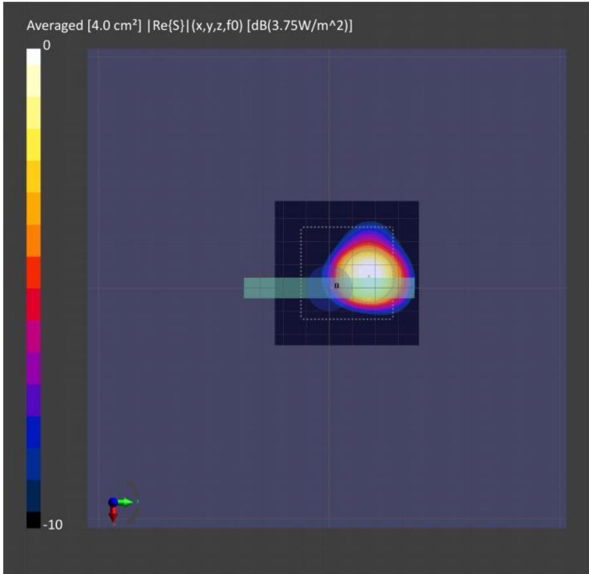
Figure 8-3: 4cm2-averaged power density distribution measured at input.power.limit of 4.44 dBm on the Back for n261 beam 15
