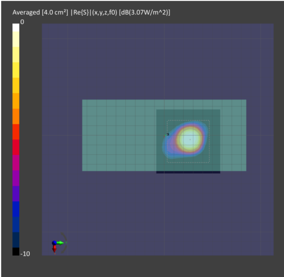
Figure 8-2: 4cm2-averaged power density distribution measured at input.power.limit of 8.5dBm on the back surface for n260 beam 1
