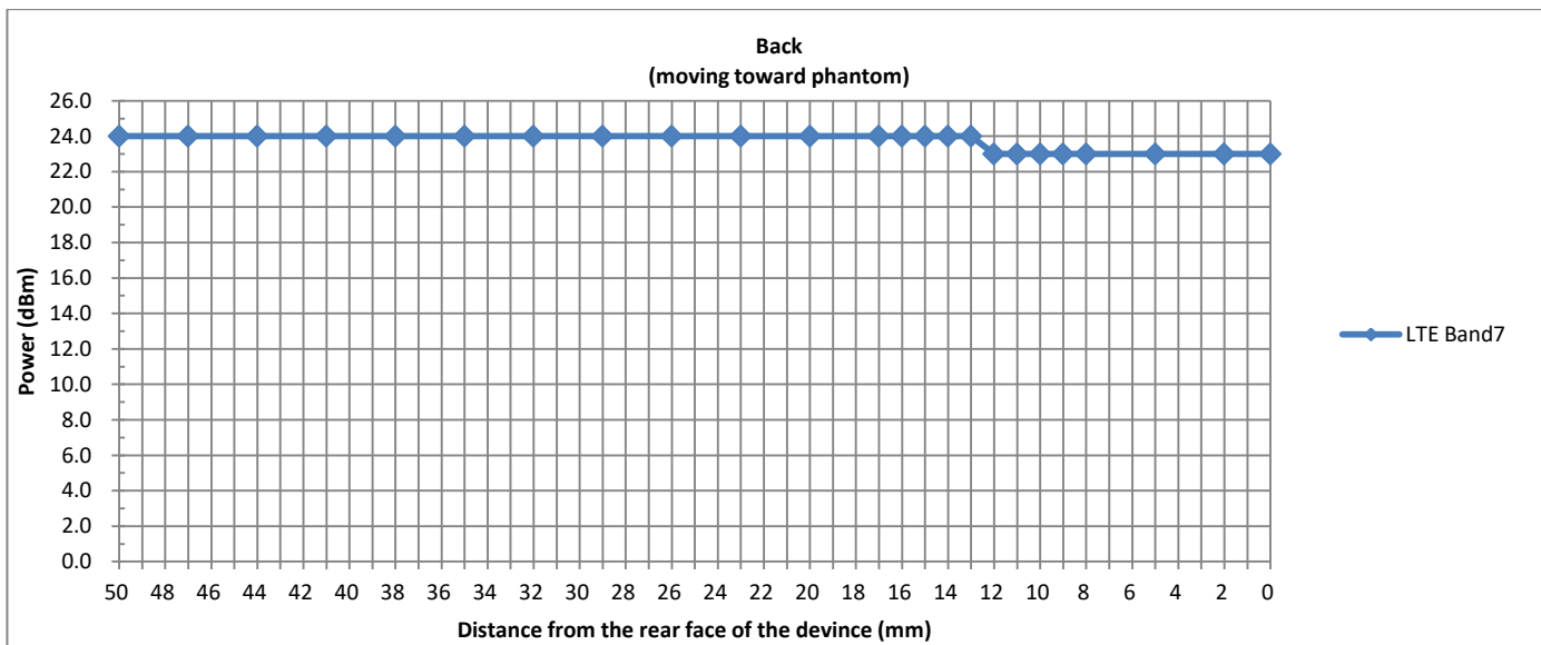
Handheld Triggering Distance (mm) and Triggering Power (dBm)
