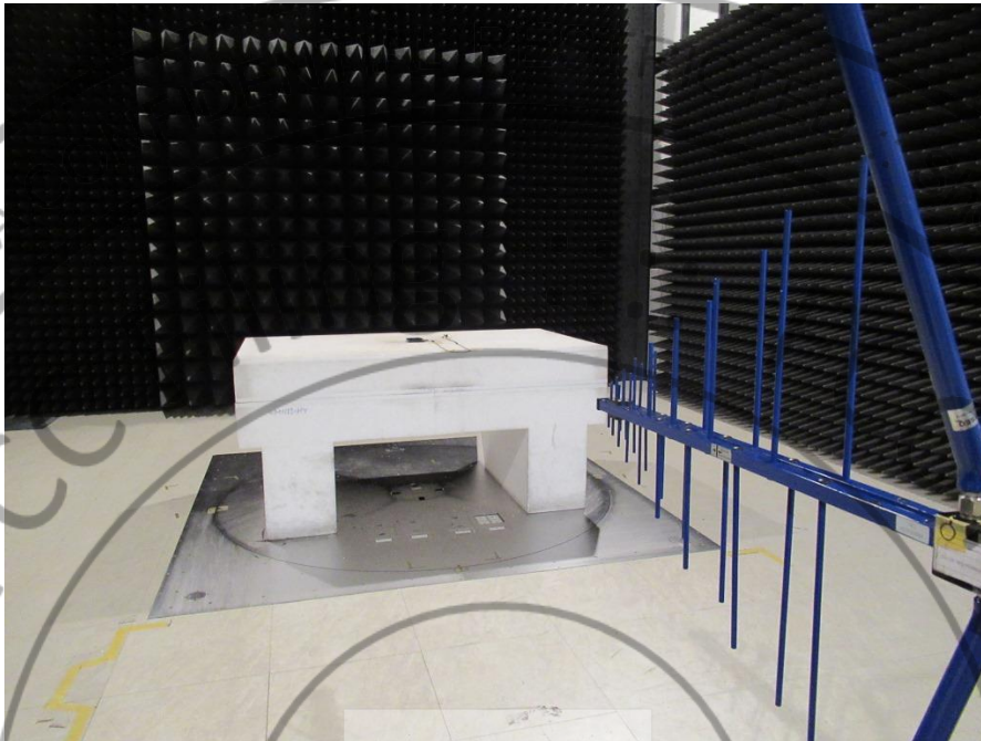
X Plane with Earphone for LTE Band 2 LF
