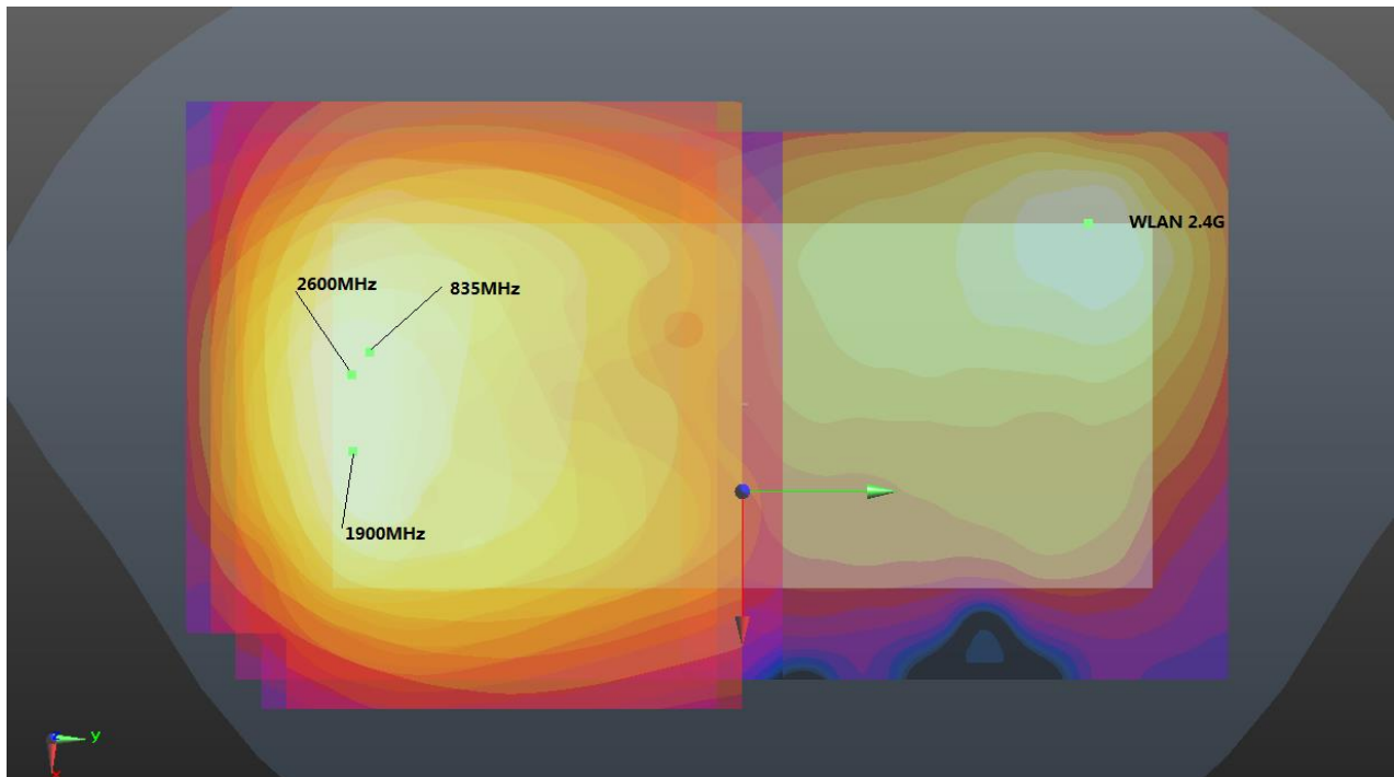
Back (0mm) + WLAN 2.4G (0mm)
