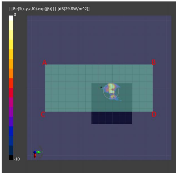
Figure 2.3.7.1-5 Measured (left) and Simulated (right) peak power density distributions for the worst case found in the back surface measurement plane for n260 ( Back module, beam 28, back surface )
