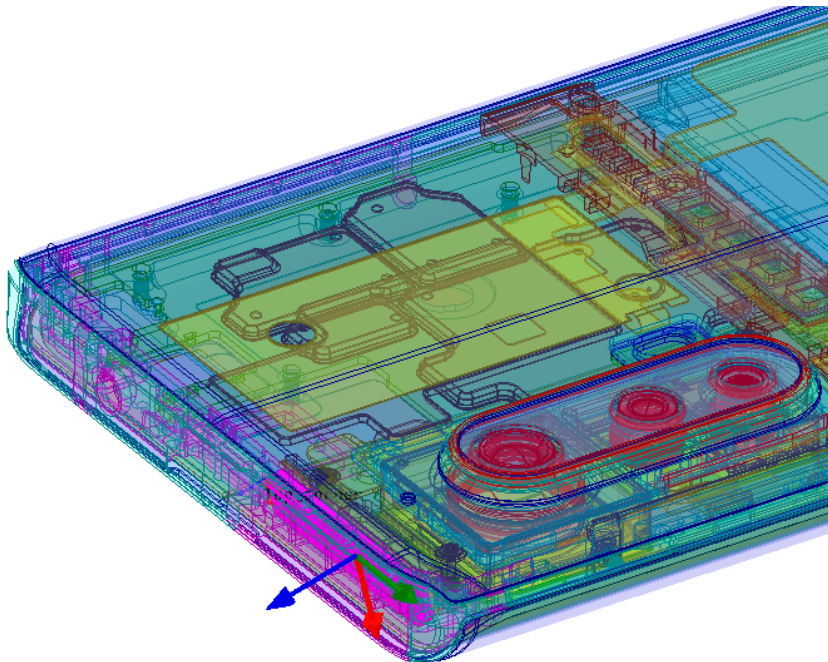
Figure 2.3.4-1: 3D model used for Module 0 (Back module), the antenna array is highlighted
