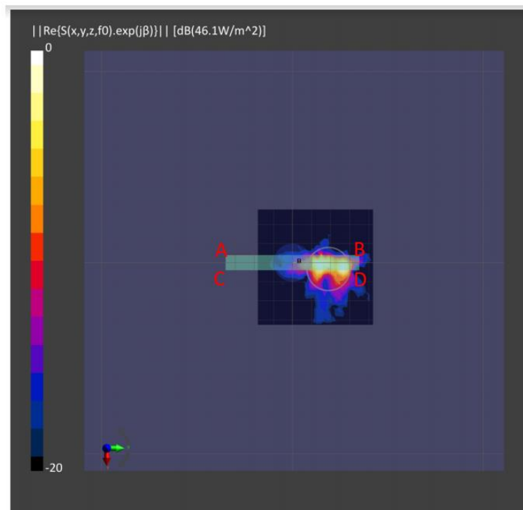
Figure 2.3.7.1-7 Measured (left) and Simulated (right) peak power density distributions for the worst case found in the Top surface measurement plane for n261 ( Top module, beam 23, Top surface )
