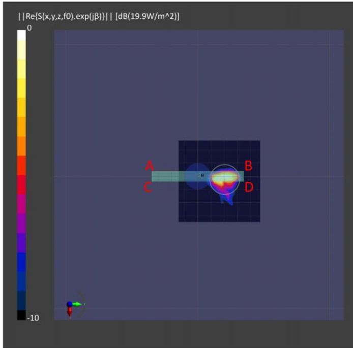
Figure 2.3.7.1-4 Measured (left) and Simulated (right) peak power density distributions for the worst case found in the Top surface measurement plane for n261 ( Top module, beam 151, Top surface )
