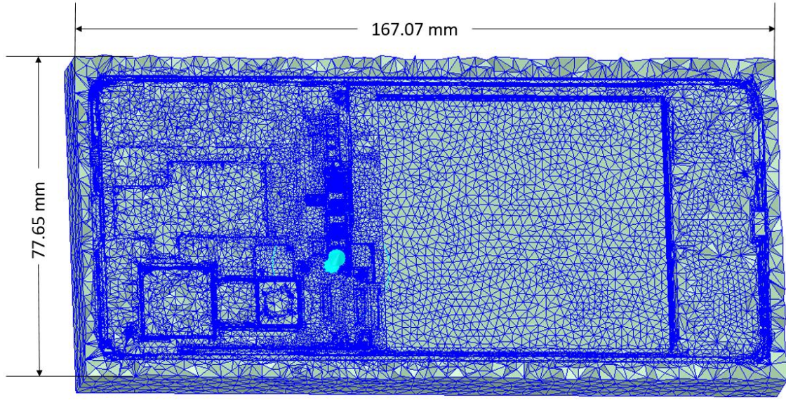
Figure 2.3.3-1: The HFSS mesh in a model of the device. After finding the simulated electric and magnetic (E and H) fields, the Poynting vector is calculated based on “peak” (i.e. non-RMS) field values in a grid with a 1 mm step, on the appropriate measurement planes as defined in previous sections. The Poynting vector at each spatial point is readily available in HFSS through the “Field Calculator” navigation option. The magnitude of the real part of the Poynting vector (all X, Y, Z components) at each spatial point i.e. the point power density is exported from HFSS to do the averaging. The spatially averaged power density at each point on a given surface is then calculated by taking the average of the point power density over a 4 square cm area. Thus the total power density (all X, Y, Z components) through any given surface is used to calculate the averaged power density.
