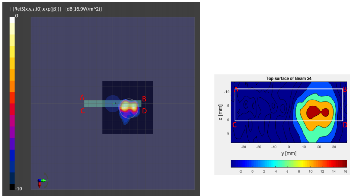
Figure 2.3.7.1-3 Measured (left) and Simulated (right) peak power density distributions for the worst case found in the Top surface measurement plane for n261 ( Top module, beam 24, Top surface )
