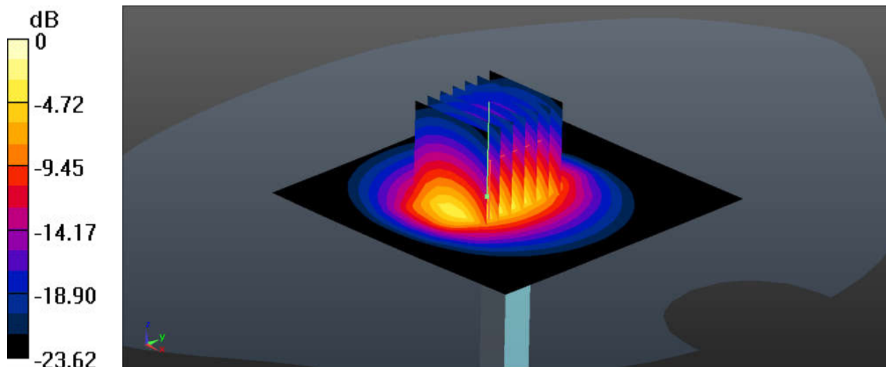
0 dB = 19.3 W/kg
