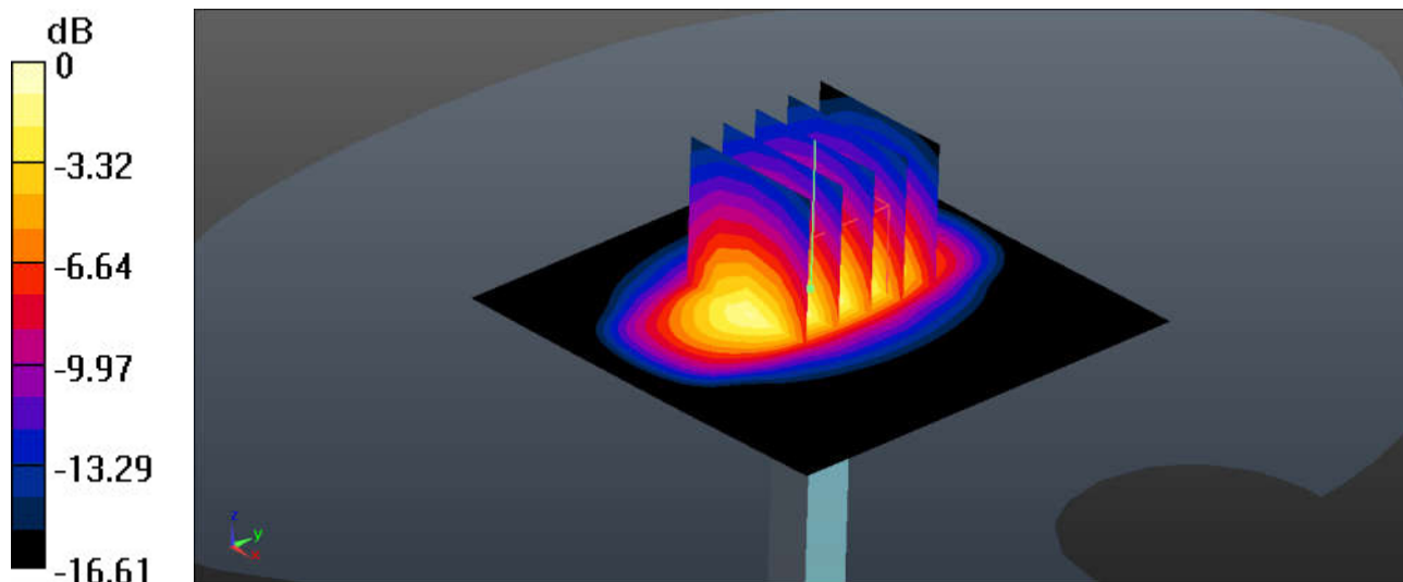
0 dB = 13.4 W/kg
