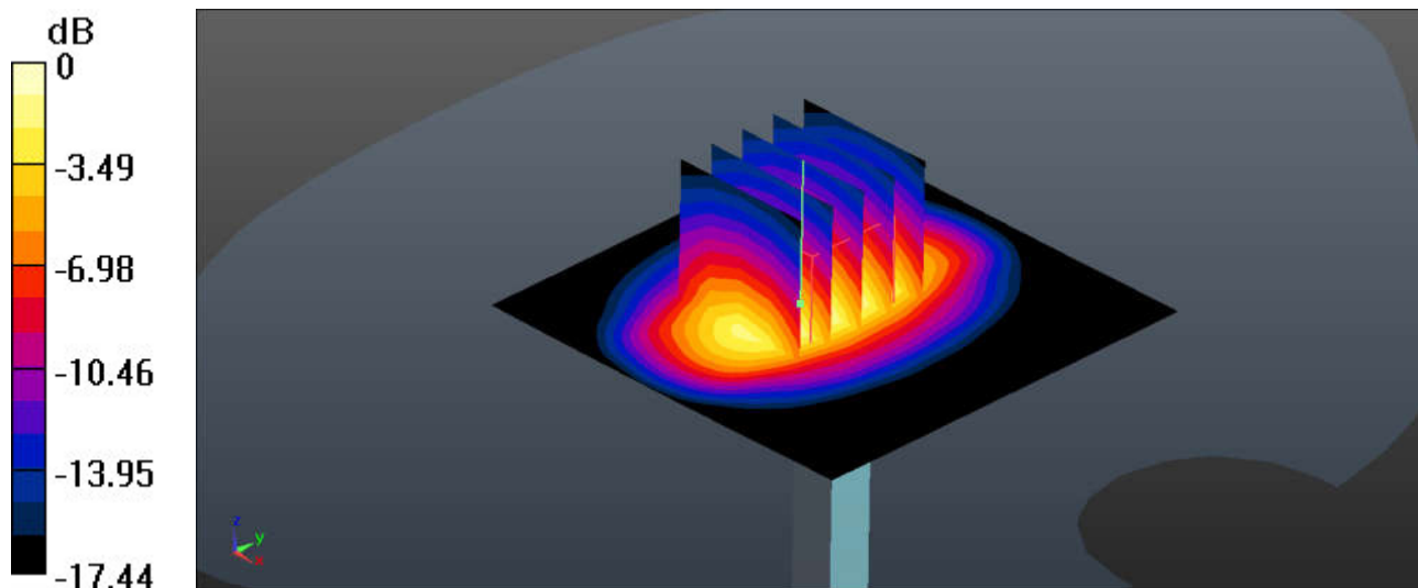
0 dB = 12.6 W/kg
