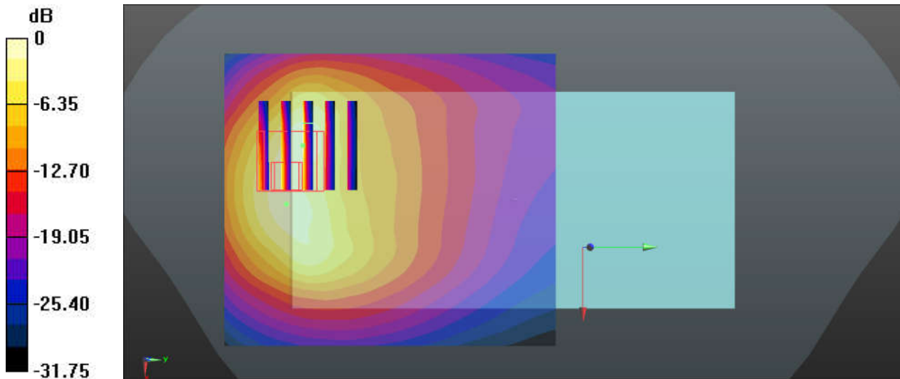
0 dB = 9.94 W/kg = 9.97 dBW/kg
