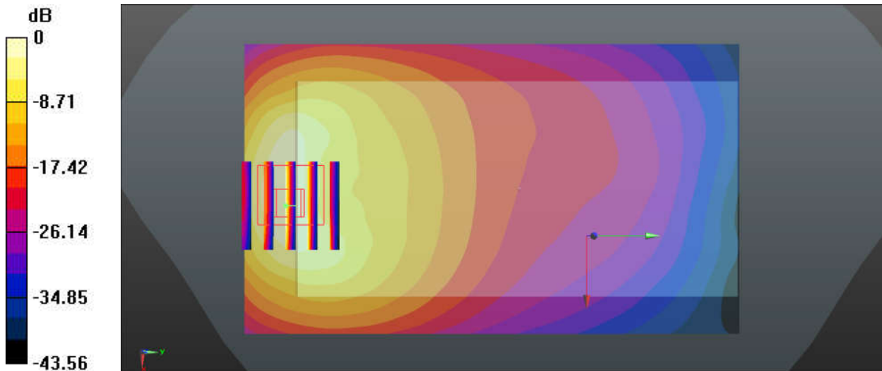
0 dB = 7.67 W/kg = 8.85 dBW/kg
