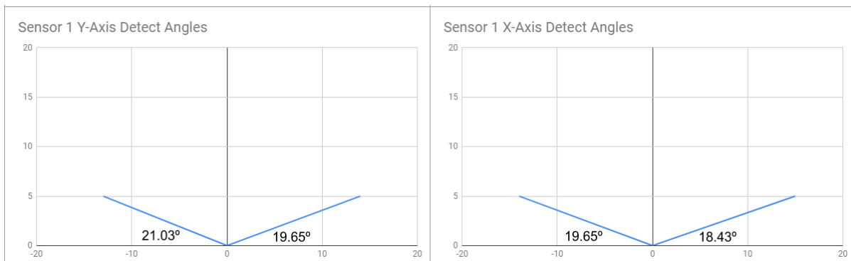
Measured angular responses of Sensor 1 at the 5 mm test separation distance.
