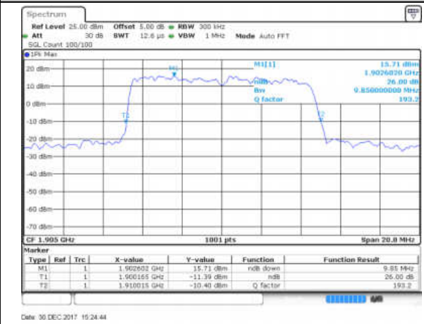
Middle Channel / 10MHz / 64QAM
