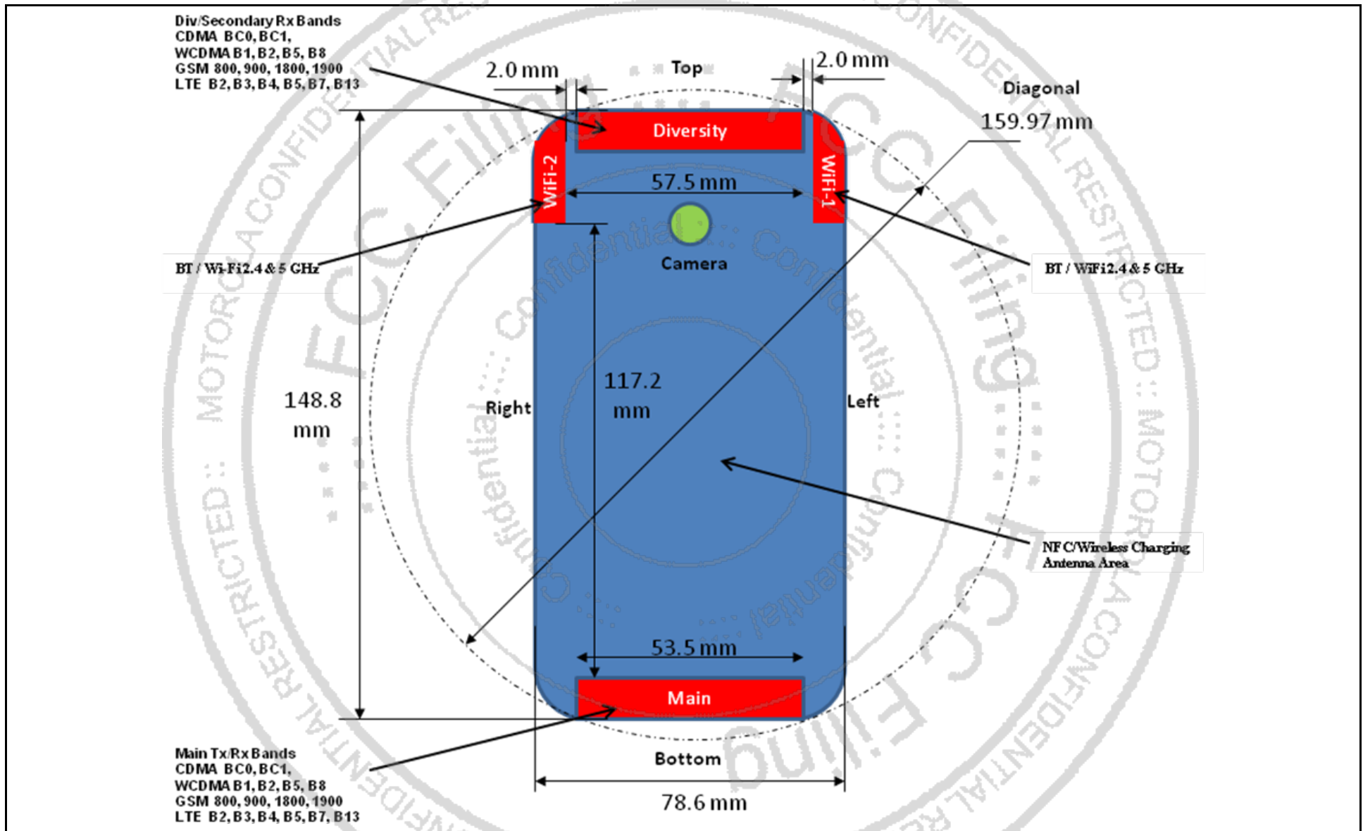
Photograph 9-5: Antenna Locations and Spacings (Viewed from Back Side).
