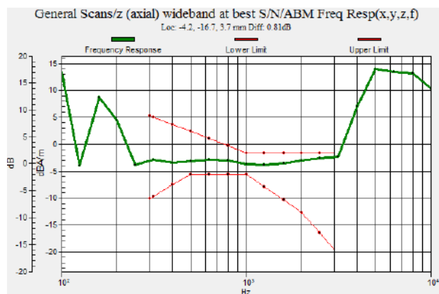
Fig 7.5 WCDMA Band II Ch1413
