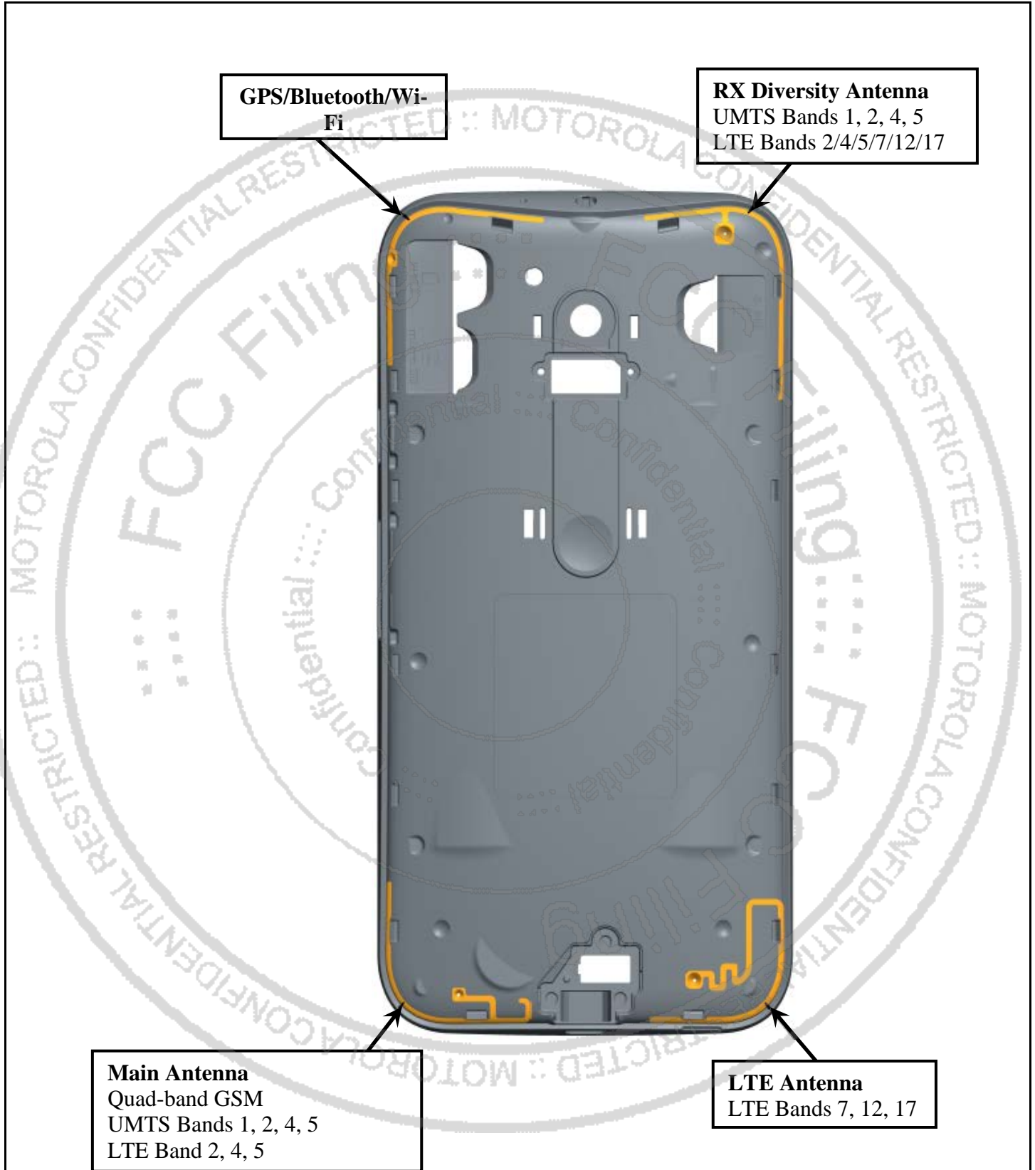
Photograph 9-6: Antenna Locations.
