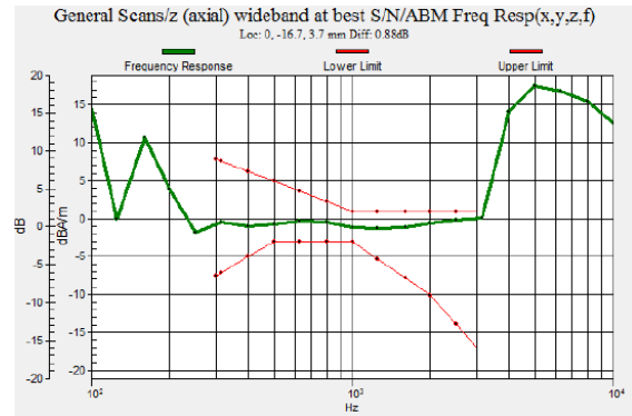
Fig 7.2 GSM1900 Ch661
