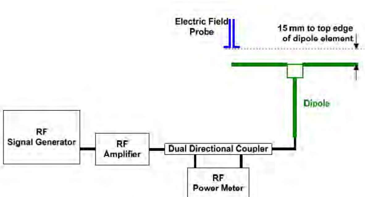
Fig. 6.1 System Validation Setup
