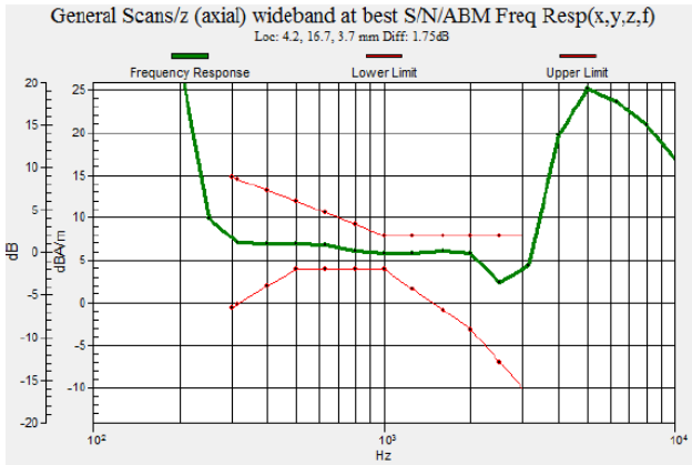
Fig 7.1 GSM1900 Ch661
