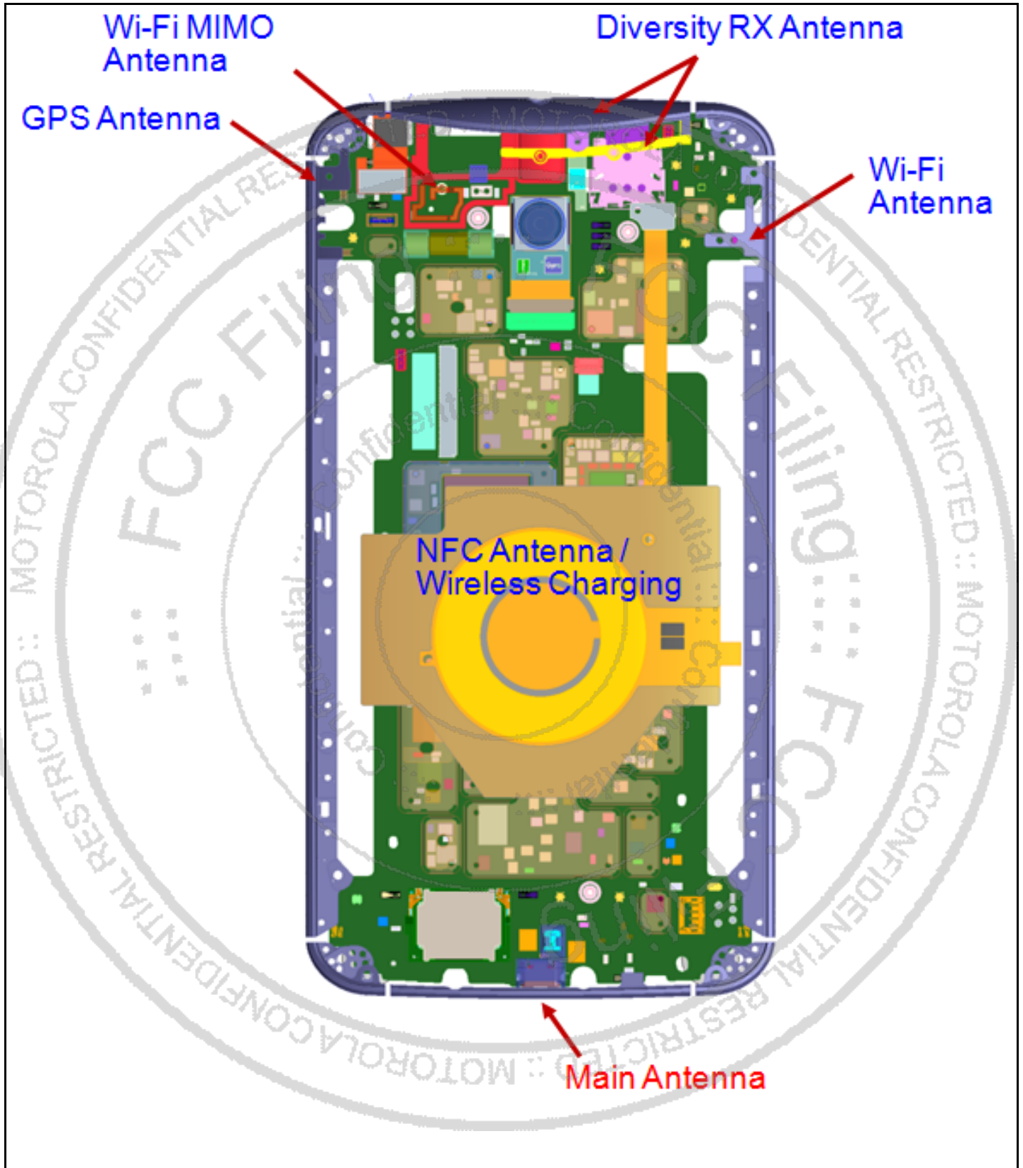
Photograph 9-4: Antenna Locations.
